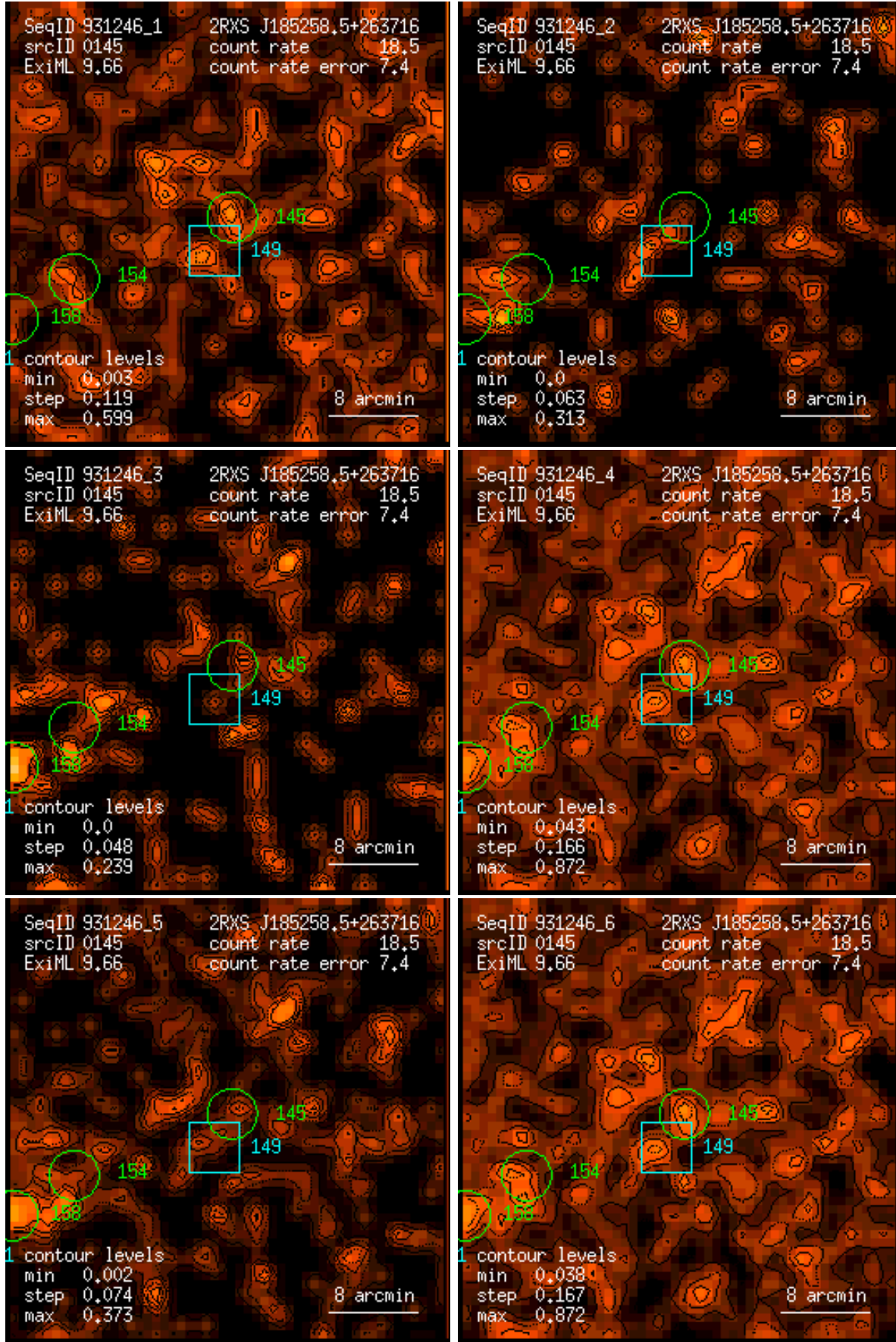
Figure 145: RASS 931246: detection 0145: band rate images, Gaussian filter: (1) PSPC channels 11 – 41, (2) 52 – 90, (3) 91 – 201, (4) 11 – 235, (5) 52 – 201, (6) 11 – 201. Broad band rates in counts/ks. Band rate contour levels in counts/ks/arcmin 2 .
