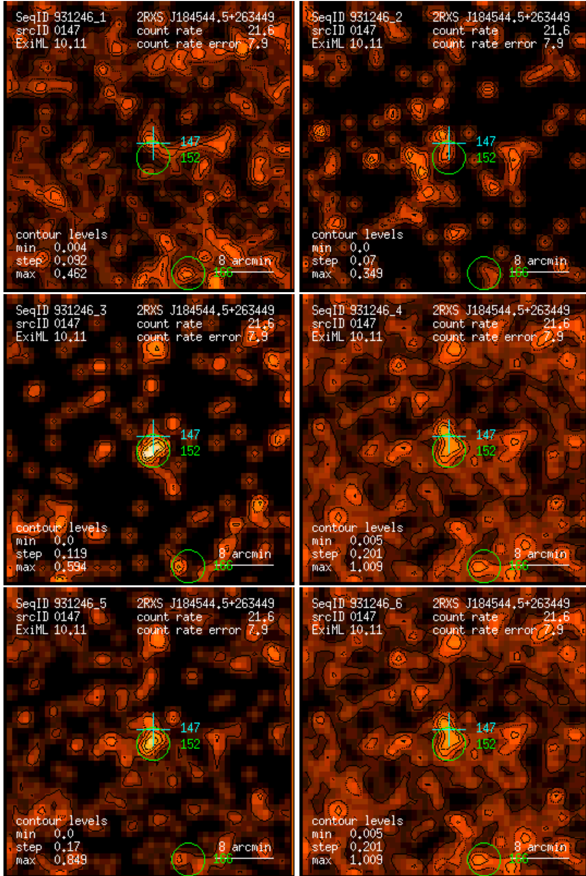
Figure 147: RASS 931246: detection 0147: band rate images, Gaussian filter: (1) PSPC channels 11 – 41, (2) 52 – 90, (3) 91 – 201, (4) 11 – 235, (5) 52 – 201, (6) 11 – 201. Broad band rates in counts/ks. Band rate contour levels in counts/ks/arcmin 2 .
