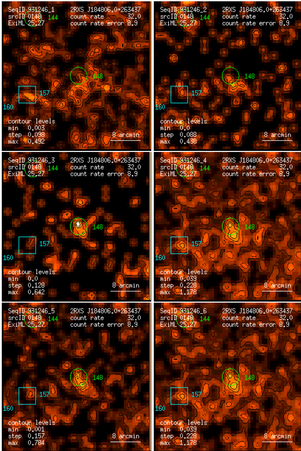
Figure 148: RASS 931246: detection 0148: band rate images, Gaussian filter: (1) PSPC channels 11 – 41, (2) 52 – 90, (3) 91 – 201, (4) 11 – 235, (5) 52 – 201, (6) 11 – 201. Broad band rates in counts/ks. Band rate contour levels in counts/ks/arcmin 2 .
