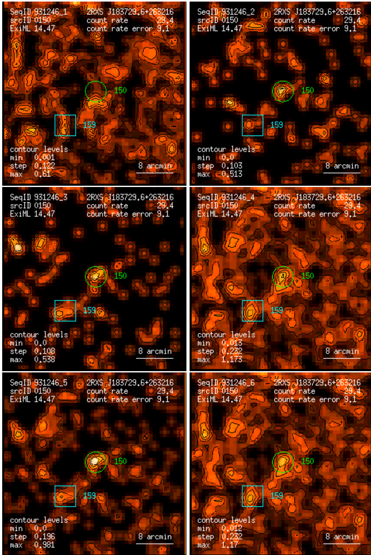
Figure 150: RASS 931246: detection 0150: band rate images, Gaussian filter: (1) PSPC channels 11 – 41, (2) 52 – 90, (3) 91 – 201, (4) 11 – 235, (5) 52 – 201, (6) 11 – 201. Broad band rates in counts/ks. Band rate contour levels in counts/ks/arcmin 2 .
