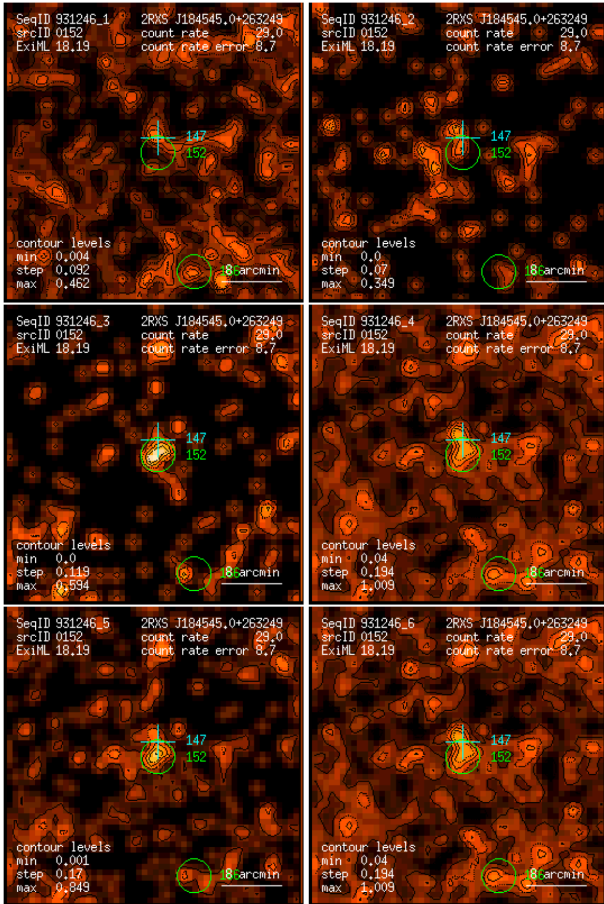
Figure 152: RASS 931246: detection 0152: band rate images, Gaussian filter: (1) PSPC channels 11 – 41, (2) 52 – 90, (3) 91 – 201, (4) 11 – 235, (5) 52 – 201, (6) 11 – 201. Broad band rates in counts/ks. Band rate contour levels in counts/ks/arcmin 2 .
