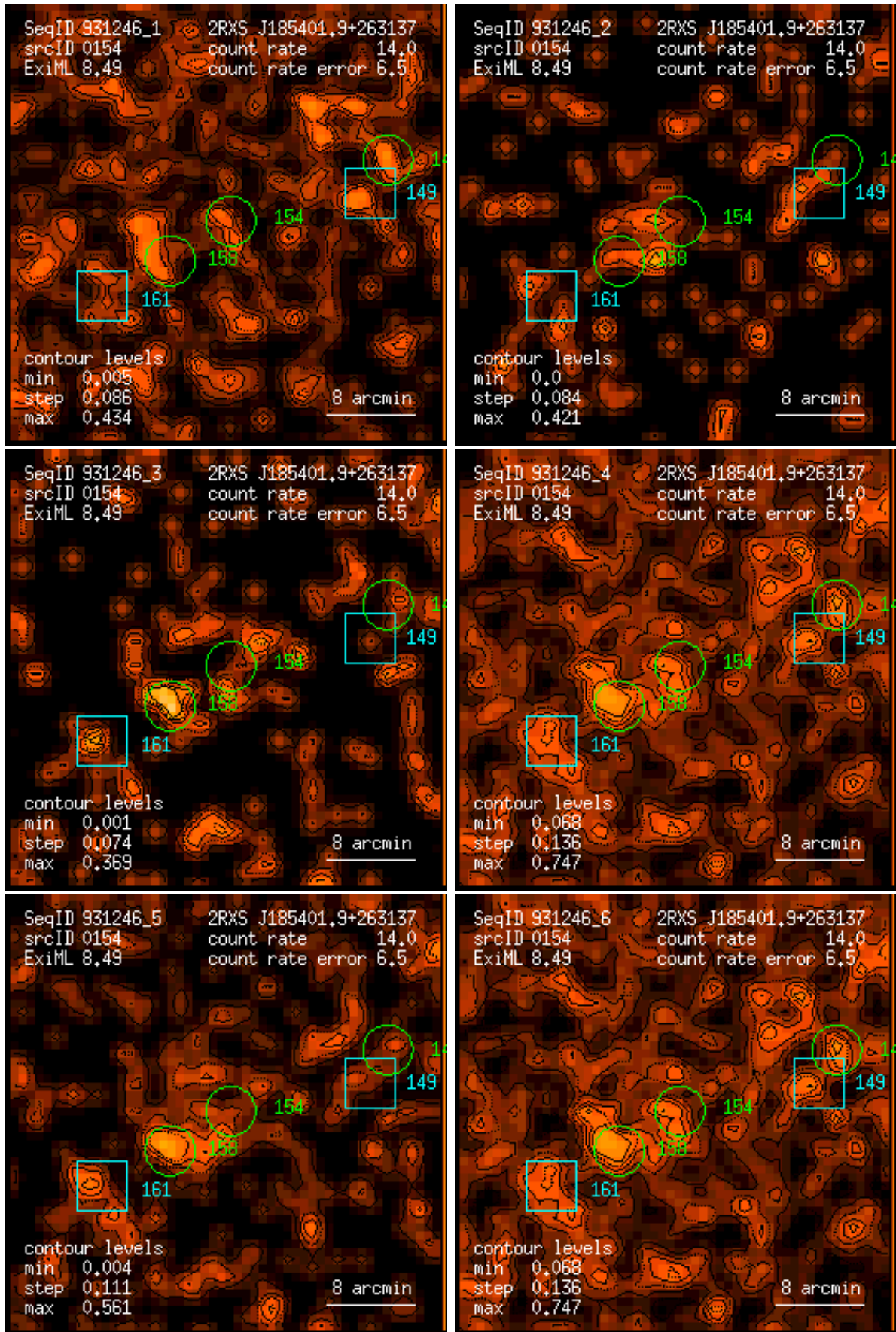
Figure 154: RASS 931246: detection 0154: band rate images, Gaussian filter: (1) PSPC channels 11 – 41, (2) 52 – 90, (3) 91 – 201, (4) 11 – 235, (5) 52 – 201, (6) 11 – 201. Broad band rates in counts/ks. Band rate contour levels in counts/ks/arcmin 2 .
