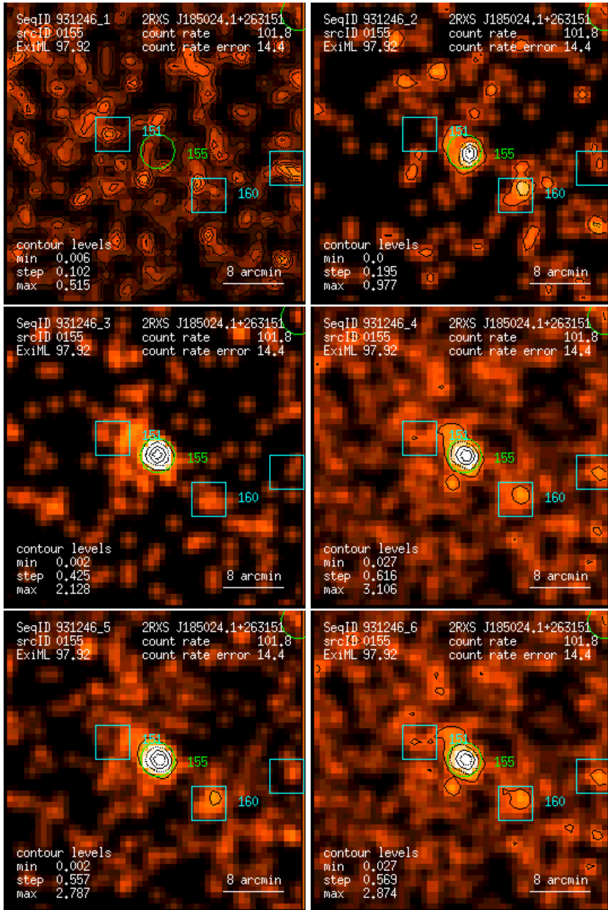
Figure 155: RASS 931246: detection 0155: band rate images, Gaussian filter: (1) PSPC channels 11 – 41, (2) 52 – 90, (3) 91 – 201, (4) 11 – 235, (5) 52 – 201, (6) 11 – 201. Broad band rates in counts/ks. Band rate contour levels in counts/ks/arcmin 2 .
