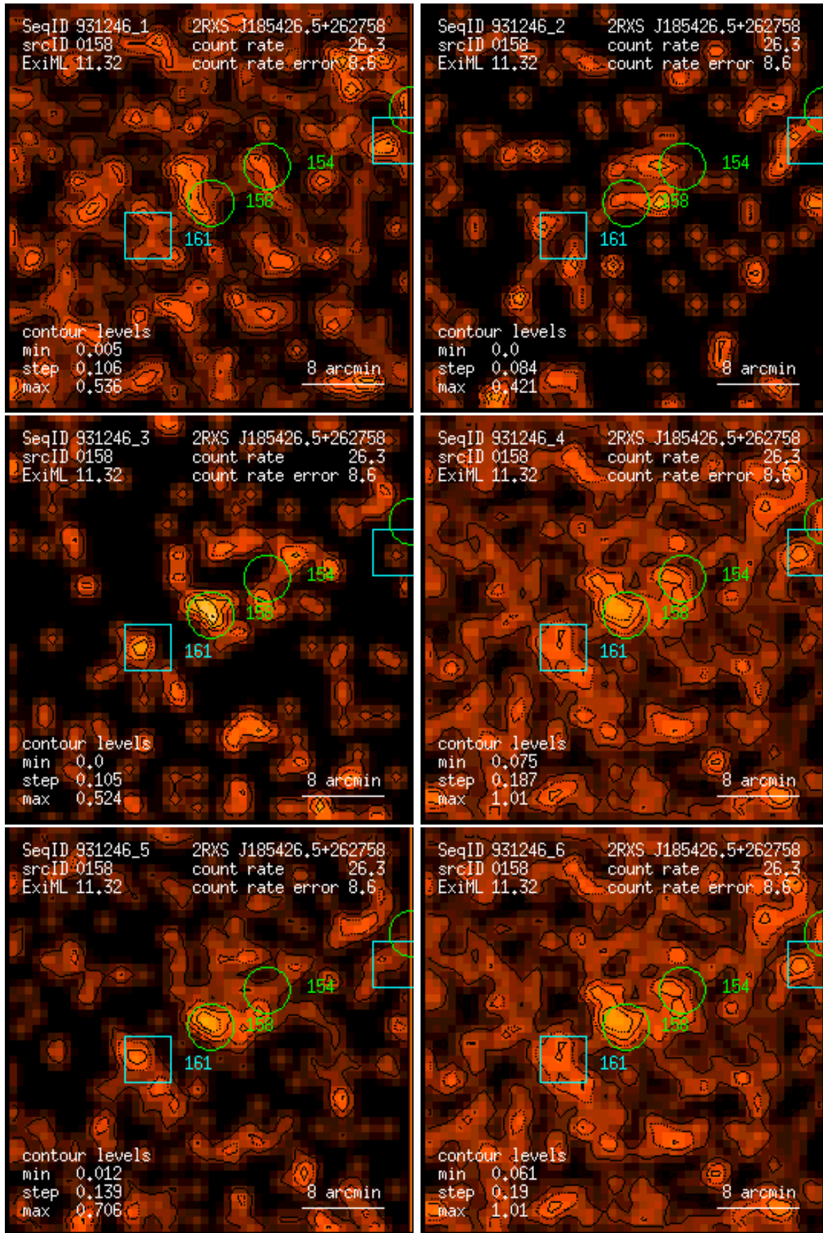
Figure 158: RASS 931246: detection 0158: band rate images, Gaussian filter: (1) PSPC channels 11 – 41, (2) 52 – 90, (3) 91 – 201, (4) 11 – 235, (5) 52 – 201, (6) 11 – 201. Broad band rates in counts/ks. Band rate contour levels in counts/ks/arcmin 2 .
