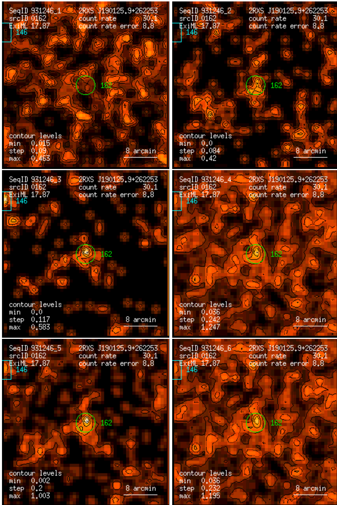
Figure 162: RASS 931246: detection 0162: band rate images, Gaussian filter: (1) PSPC channels 11 – 41, (2) 52 – 90, (3) 91 – 201, (4) 11 – 235, (5) 52 – 201, (6) 11 – 201. Broad band rates in counts/ks. Band rate contour levels in counts/ks/arcmin 2 .
