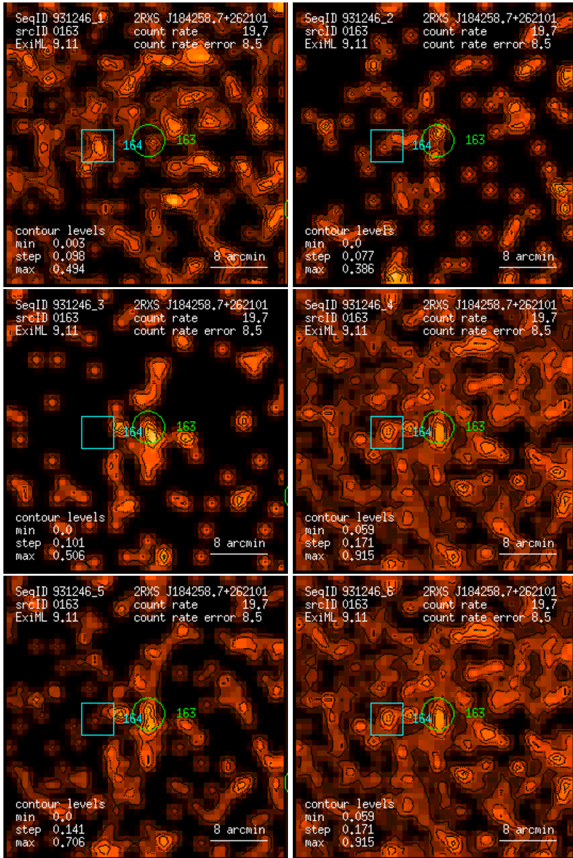
Figure 163: RASS 931246: detection 0163: band rate images, Gaussian filter: (1) PSPC channels 11 – 41, (2) 52 – 90, (3) 91 – 201, (4) 11 – 235, (5) 52 – 201, (6) 11 – 201. Broad band rates in counts/ks. Band rate contour levels in counts/ks/arcmin 2 .
