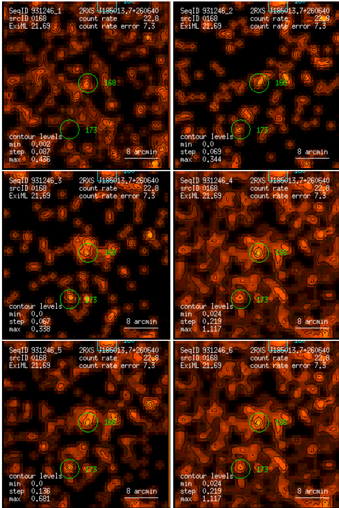
Figure 168: RASS 931246: detection 0168: band rate images, Gaussian filter: (1) PSPC channels 11 – 41, (2) 52 – 90, (3) 91 – 201, (4) 11 – 235, (5) 52 – 201, (6) 11 – 201. Broad band rates in counts/ks. Band rate contour levels in counts/ks/arcmin 2 .
