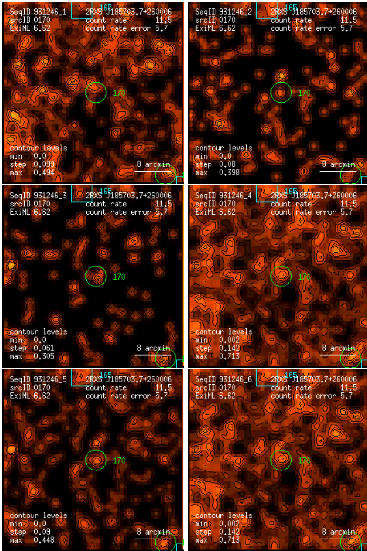
Figure 170: RASS 931246: detection 0170: band rate images, Gaussian filter: (1) PSPC channels 11 – 41, (2) 52 – 90, (3) 91 – 201, (4) 11 – 235, (5) 52 – 201, (6) 11 – 201. Broad band rates in counts/ks. Band rate contour levels in counts/ks/arcmin 2 .
