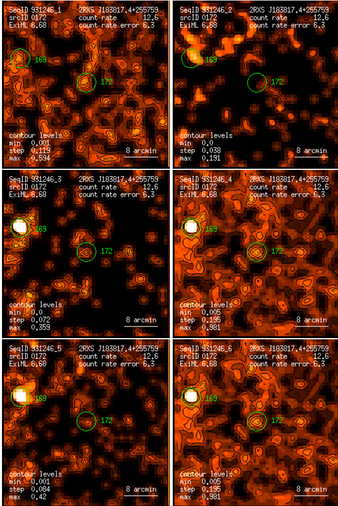
Figure 172: RASS 931246: detection 0172: band rate images, Gaussian filter: (1) PSPC channels 11 – 41, (2) 52 – 90, (3) 91 – 201, (4) 11 – 235, (5) 52 – 201, (6) 11 – 201. Broad band rates in counts/ks. Band rate contour levels in counts/ks/arcmin 2 .
