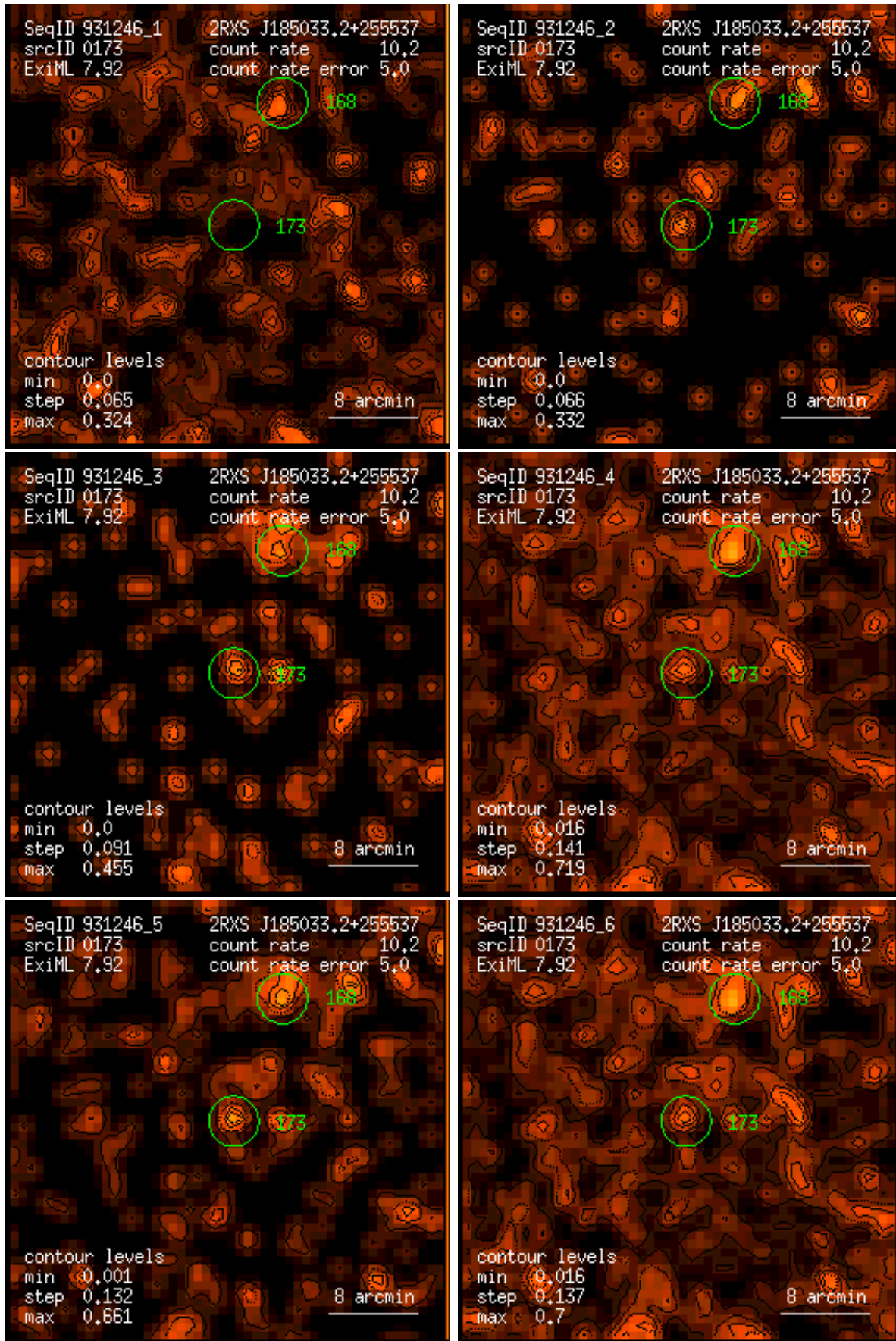
Figure 173: RASS 931246: detection 0173: band rate images, Gaussian filter: (1) PSPC channels 11 – 41, (2) 52 – 90, (3) 91 – 201, (4) 11 – 235, (5) 52 – 201, (6) 11 – 201. Broad band rates in counts/ks. Band rate contour levels in counts/ks/arcmin 2 .
