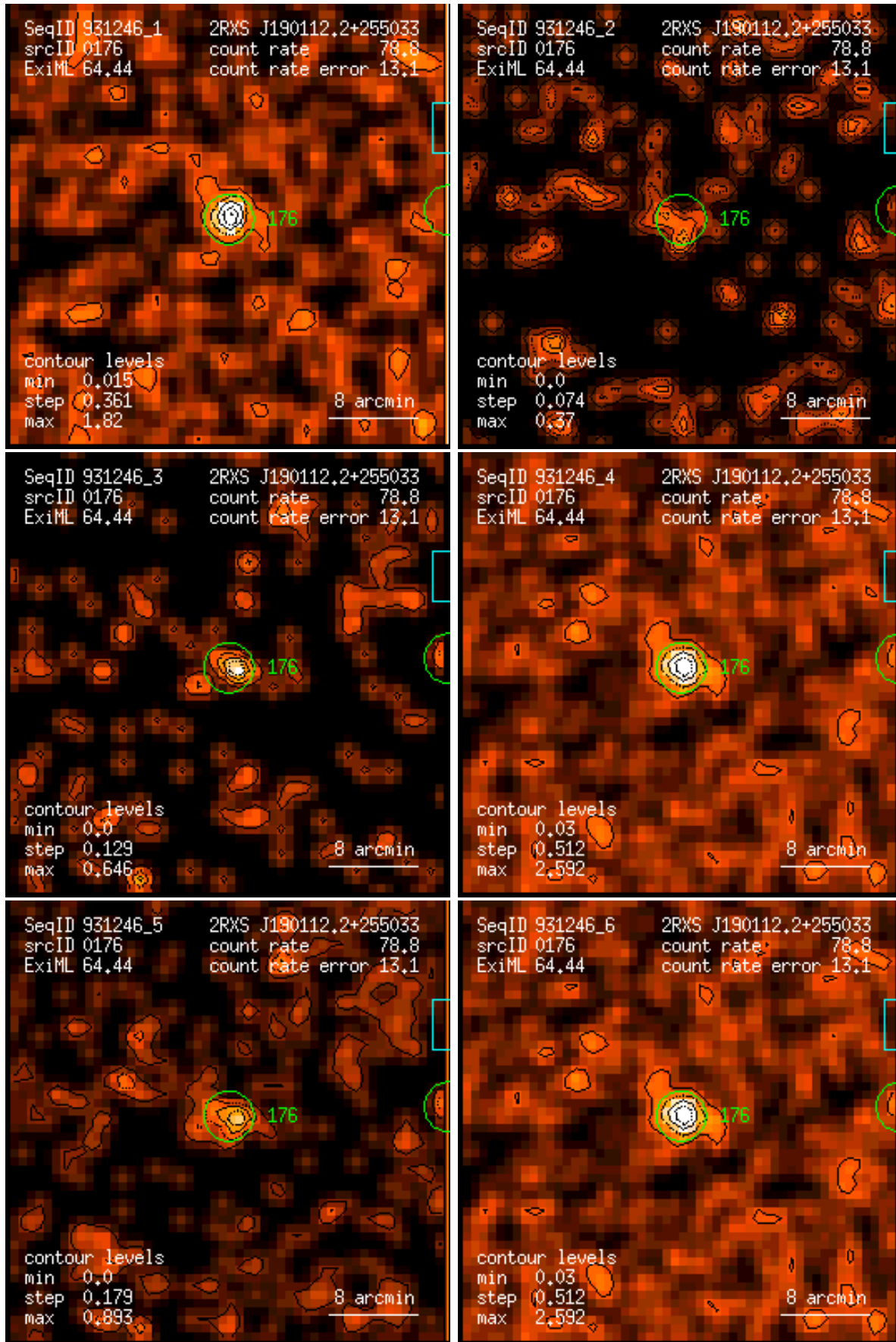
Figure 176: RASS 931246: detection 0176: band rate images, Gaussian filter: (1) PSPC channels 11 – 41, (2) 52 – 90, (3) 91 – 201, (4) 11 – 235, (5) 52 – 201, (6) 11 – 201. Broad band rates in counts/ks. Band rate contour levels in counts/ks/arcmin 2 .
