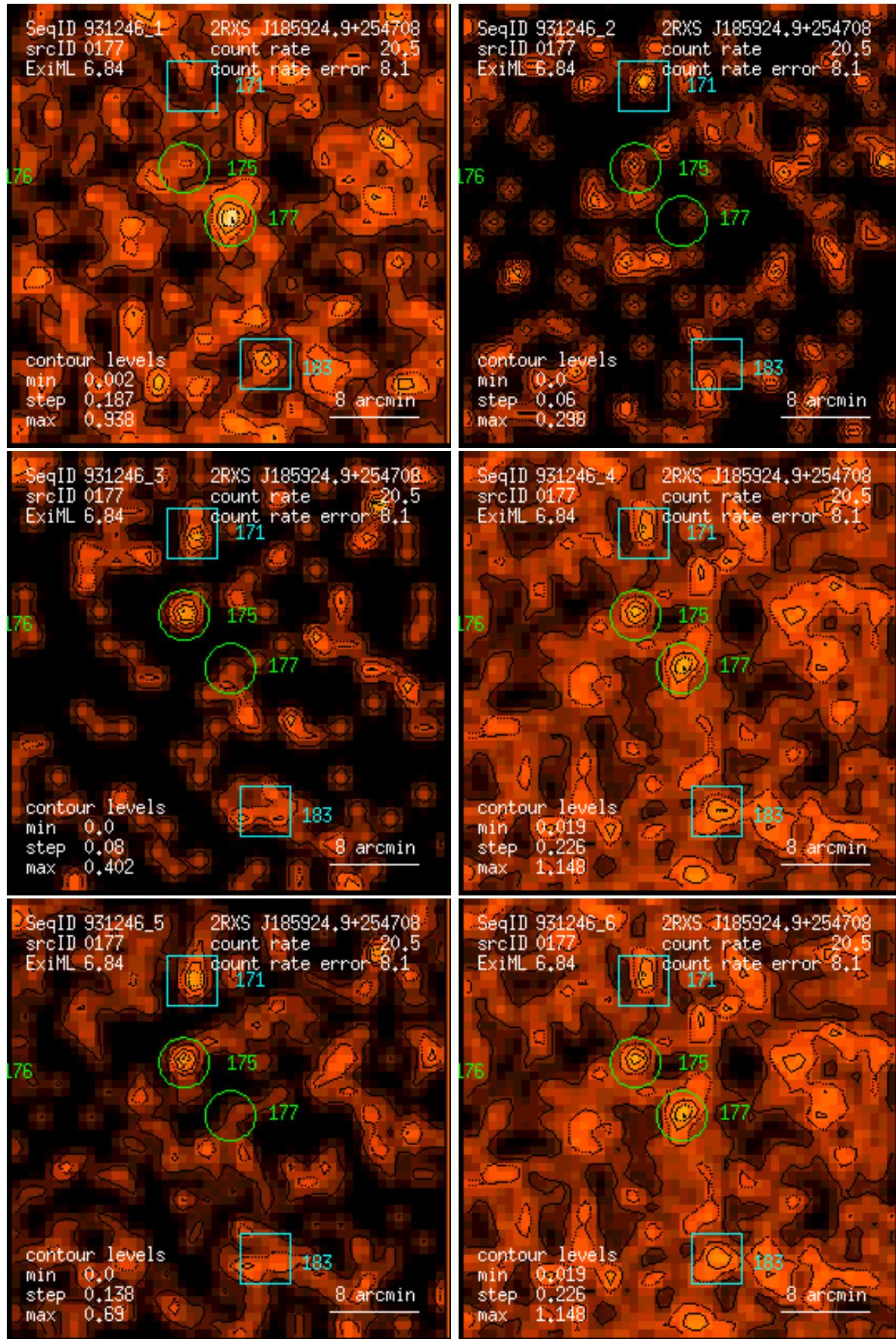
Figure 177: RASS 931246: detection 0177: band rate images, Gaussian filter: (1) PSPC channels 11 – 41, (2) 52 – 90, (3) 91 – 201, (4) 11 – 235, (5) 52 – 201, (6) 11 – 201. Broad band rates in counts/ks. Band rate contour levels in counts/ks/arcmin 2 .
