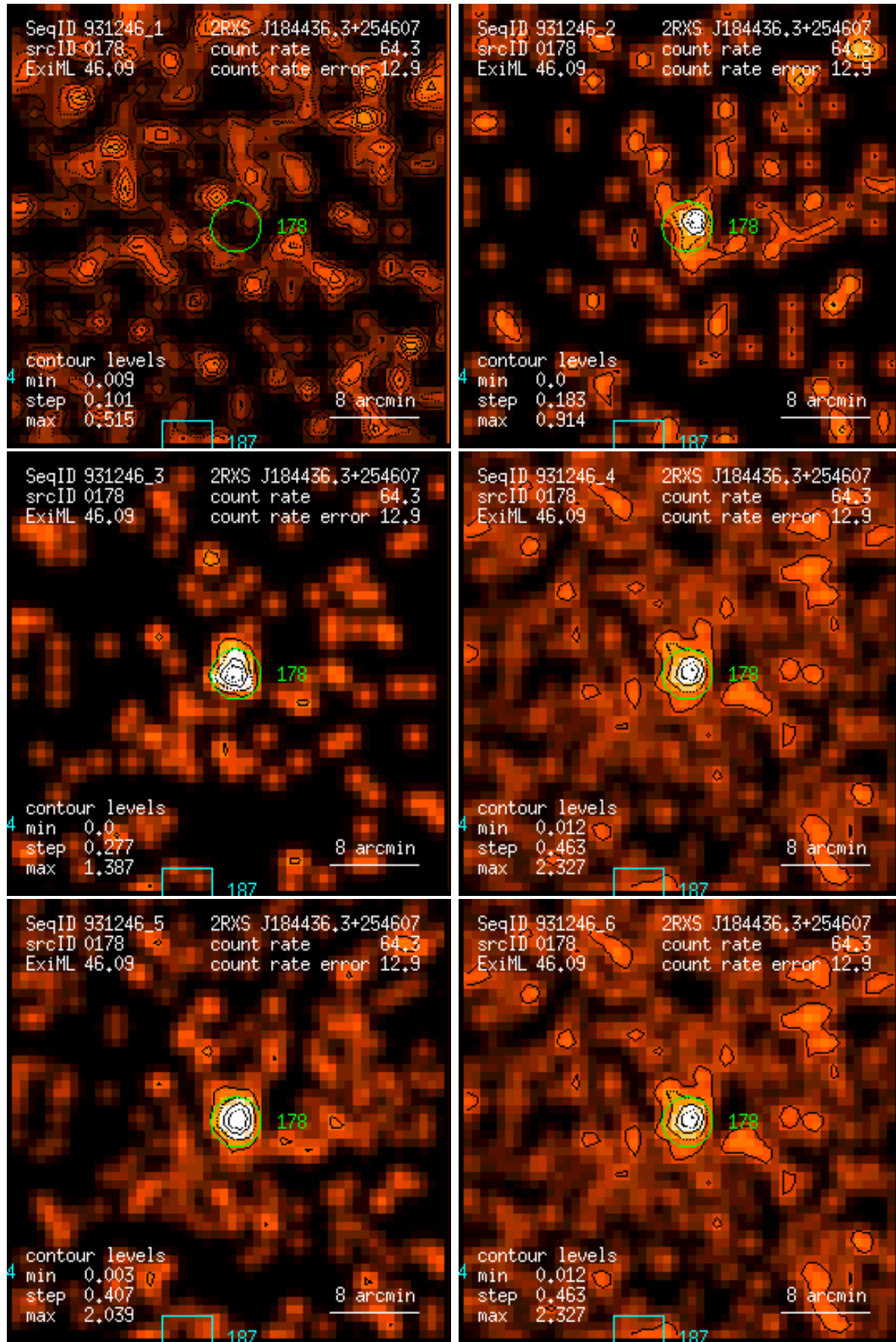
Figure 178: RASS 931246: detection 0178: band rate images, Gaussian filter: (1) PSPC channels 11 – 41, (2) 52 – 90, (3) 91 – 201, (4) 11 – 235, (5) 52 – 201, (6) 11 – 201. Broad band rates in counts/ks. Band rate contour levels in counts/ks/arcmin 2 .
