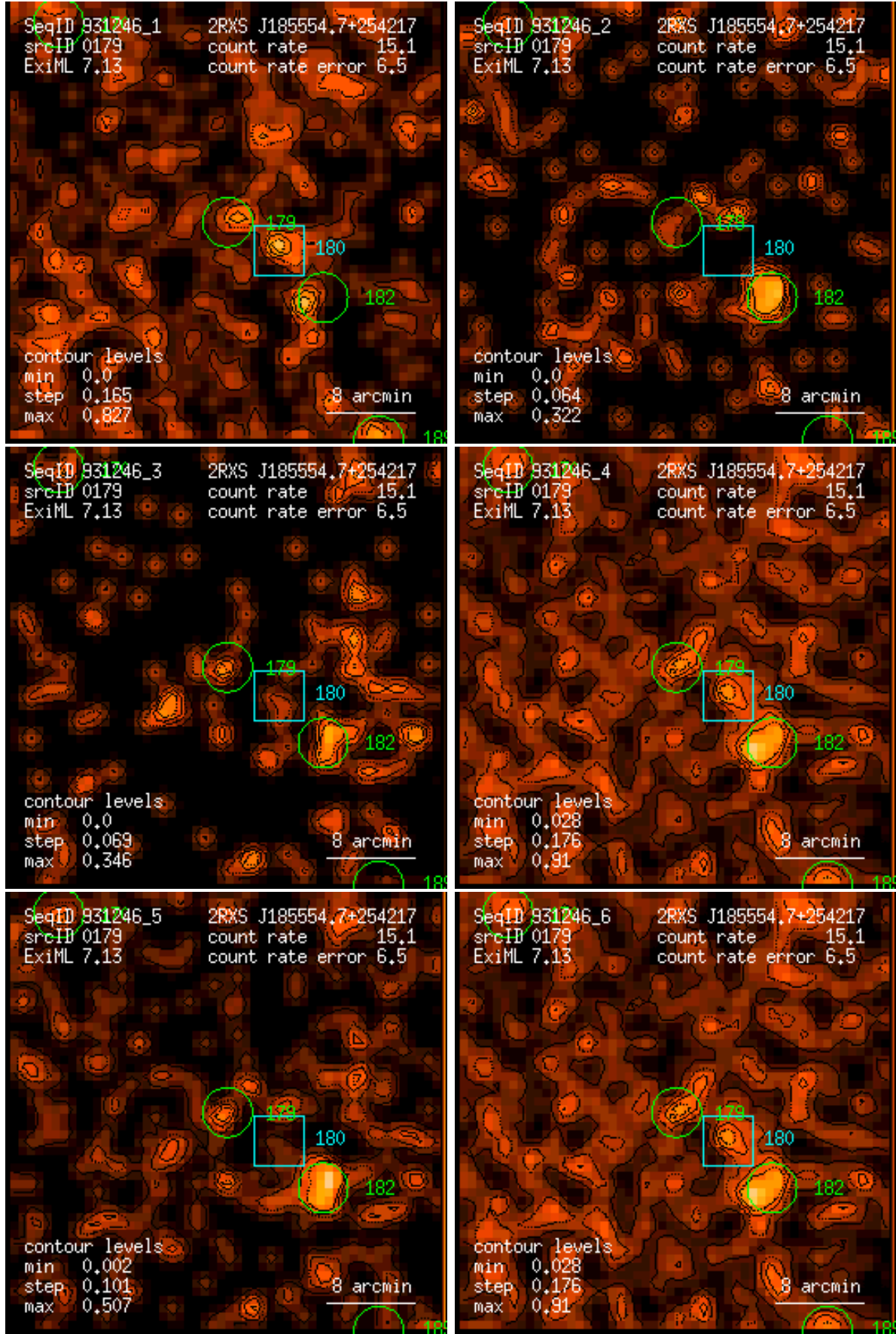
Figure 179: RASS 931246: detection 0179: band rate images, Gaussian filter: (1) PSPC channels 11 – 41, (2) 52 – 90, (3) 91 – 201, (4) 11 – 235, (5) 52 – 201, (6) 11 – 201. Broad band rates in counts/ks. Band rate contour levels in counts/ks/arcmin 2 .
