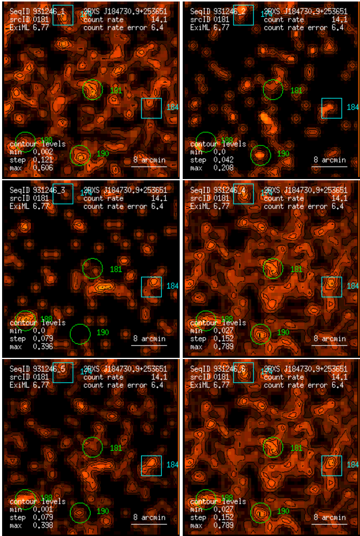
Figure 181: RASS 931246: detection 0181: band rate images, Gaussian filter: (1) PSPC channels 11 – 41, (2) 52 – 90, (3) 91 – 201, (4) 11 – 235, (5) 52 – 201, (6) 11 – 201. Broad band rates in counts/ks. Band rate contour levels in counts/ks/arcmin 2 .
