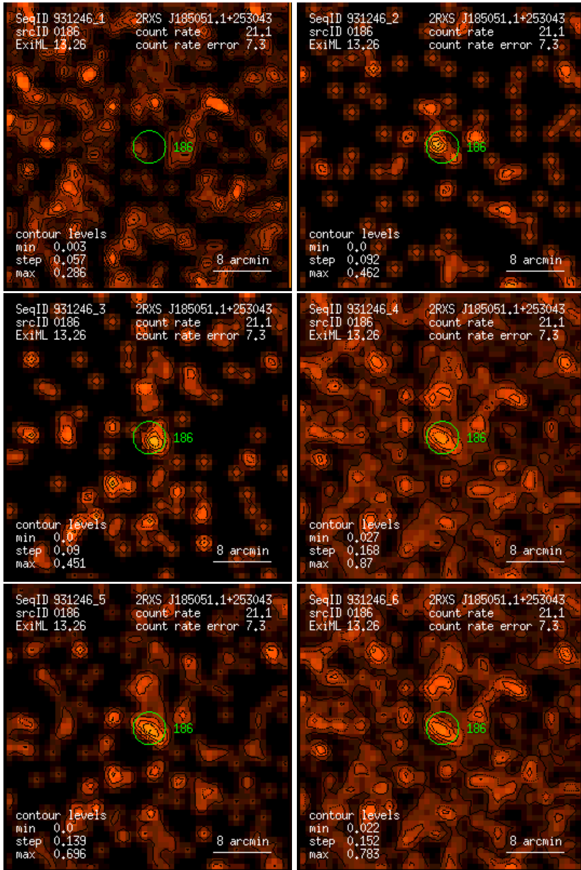
Figure 186: RASS 931246: detection 0186: band rate images, Gaussian filter: (1) PSPC channels 11 – 41, (2) 52 – 90, (3) 91 – 201, (4) 11 – 235, (5) 52 – 201, (6) 11 – 201. Broad band rates in counts/ks. Band rate contour levels in counts/ks/arcmin 2 .
