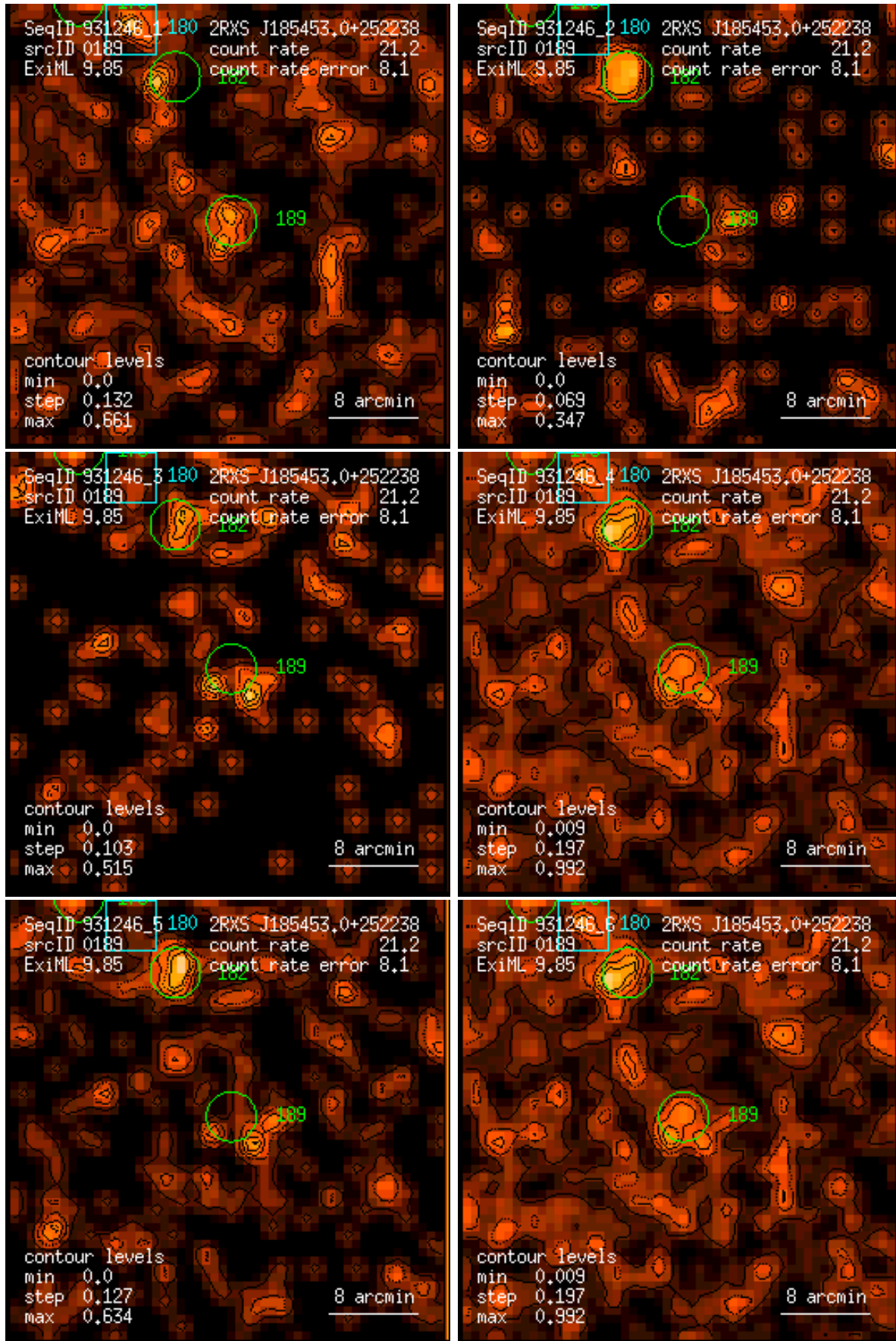
Figure 189: RASS 931246: detection 0189: band rate images, Gaussian filter: (1) PSPC channels 11 – 41, (2) 52 – 90, (3) 91 – 201, (4) 11 – 235, (5) 52 – 201, (6) 11 – 201. Broad band rates in counts/ks. Band rate contour levels in counts/ks/arcmin 2 .
