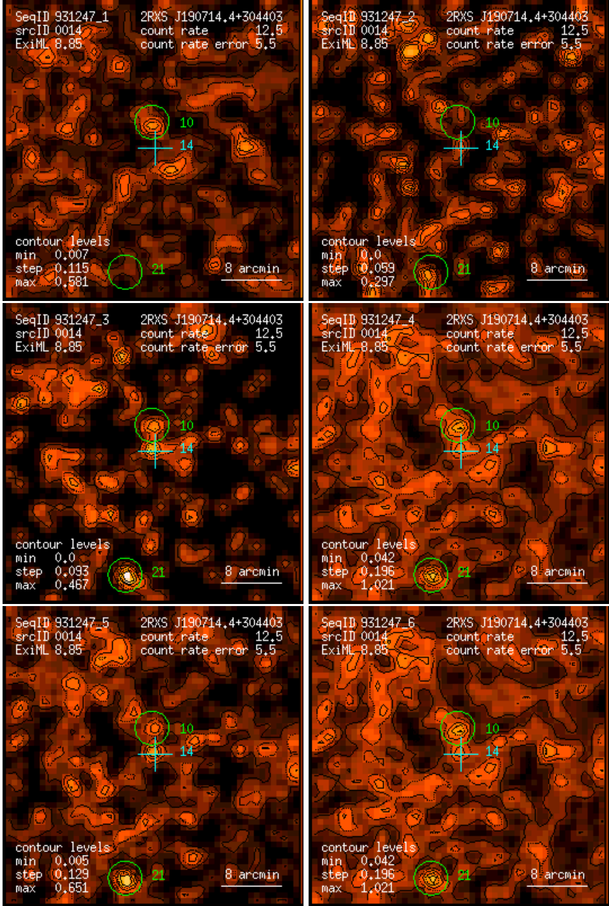
Figure 14: RASS 931247: detection 0014: band rate images, Gaussian filter: (1) PSPC channels 11 – 41, (2) 52 – 90, (3) 91 – 201, (4) 11 – 235, (5) 52 – 201, (6) 11 – 201. Broad band rates in counts/ks. Band rate contour levels in counts/ks/arcmin 2 .
