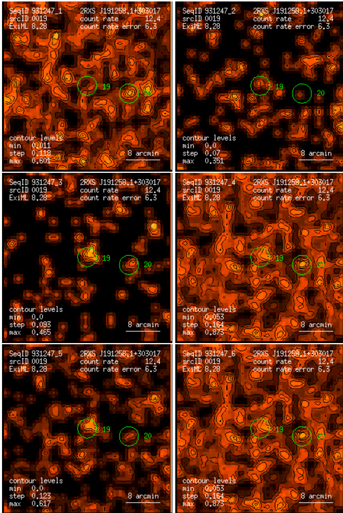
Figure 19: RASS 931247: detection 0019: band rate images, Gaussian filter: (1) PSPC channels 11 – 41, (2) 52 – 90, (3) 91 – 201, (4) 11 – 235, (5) 52 – 201, (6) 11 – 201. Broad band rates in counts/ks. Band rate contour levels in counts/ks/arcmin 2 .
