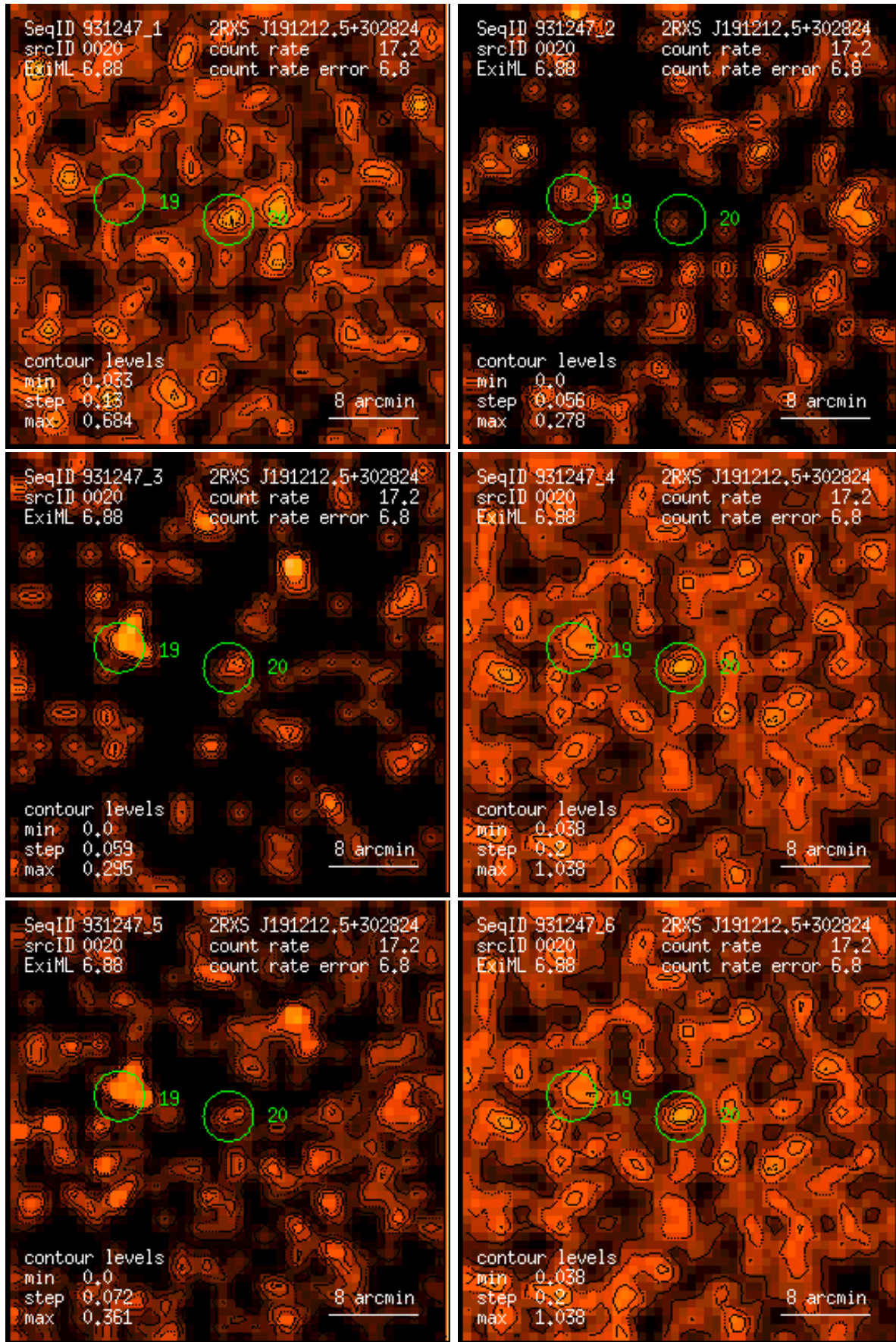
Figure 20: RASS 931247: detection 0020: band rate images, Gaussian filter: (1) PSPC channels 11 – 41, (2) 52 – 90, (3) 91 – 201, (4) 11 – 235, (5) 52 – 201, (6) 11 – 201. Broad band rates in counts/ks. Band rate contour levels in counts/ks/arcmin 2 .
