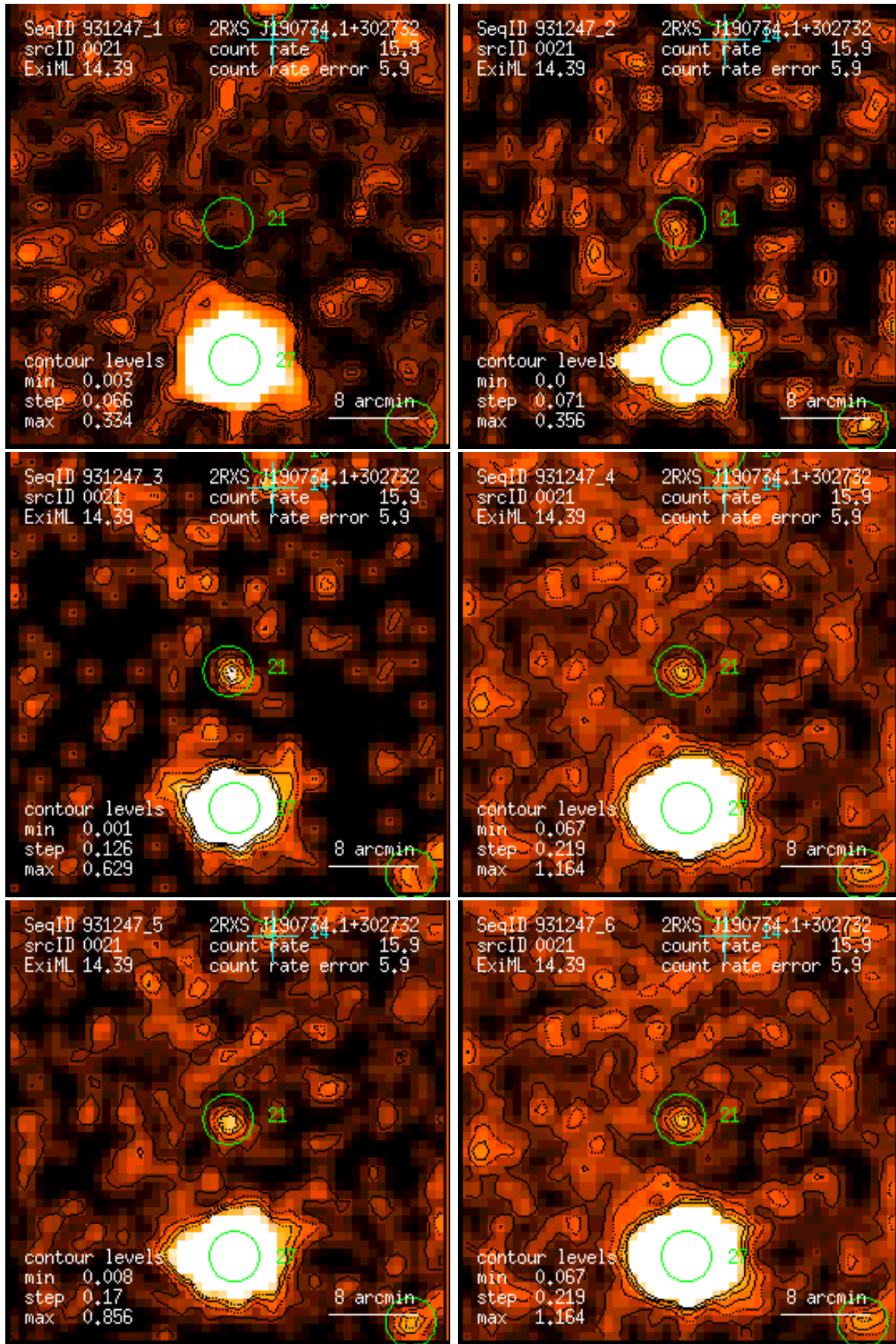
Figure 21: RASS 931247: detection 0021: band rate images, Gaussian filter: (1) PSPC channels 11 – 41, (2) 52 – 90, (3) 91 – 201, (4) 11 – 235, (5) 52 – 201, (6) 11 – 201. Broad band rates in counts/ks. Band rate contour levels in counts/ks/arcmin 2 .
