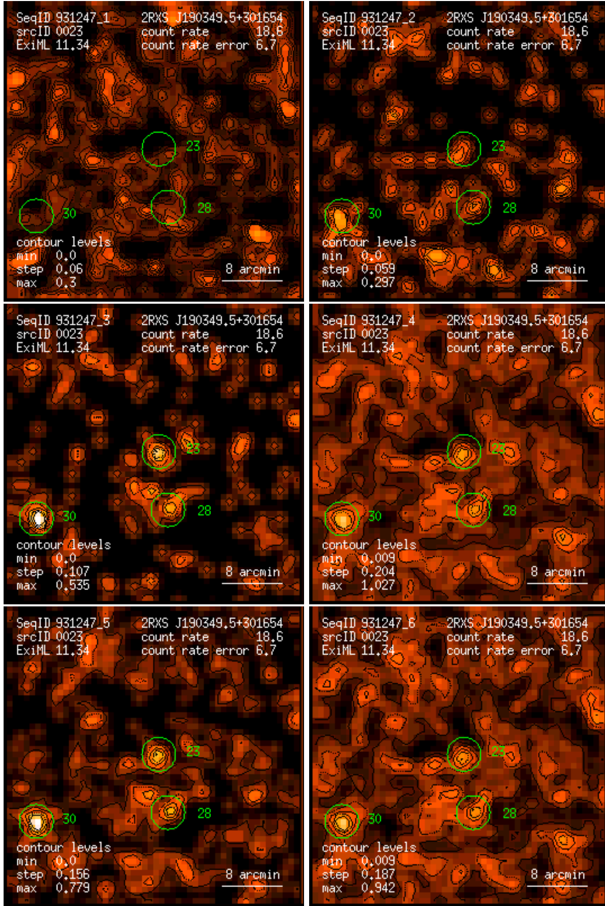
Figure 23: RASS 931247: detection 0023: band rate images, Gaussian filter: (1) PSPC channels 11 – 41, (2) 52 – 90, (3) 91 – 201, (4) 11 – 235, (5) 52 – 201, (6) 11 – 201. Broad band rates in counts/ks. Band rate contour levels in counts/ks/arcmin 2 .
