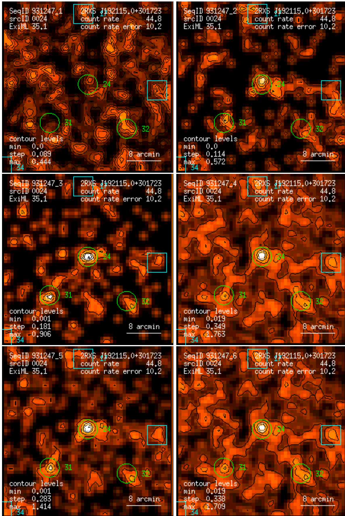
Figure 24: RASS 931247: detection 0024: band rate images, Gaussian filter: (1) PSPC channels 11 – 41, (2) 52 – 90, (3) 91 – 201, (4) 11 – 235, (5) 52 – 201, (6) 11 – 201. Broad band rates in counts/ks. Band rate contour levels in counts/ks/arcmin 2 .
