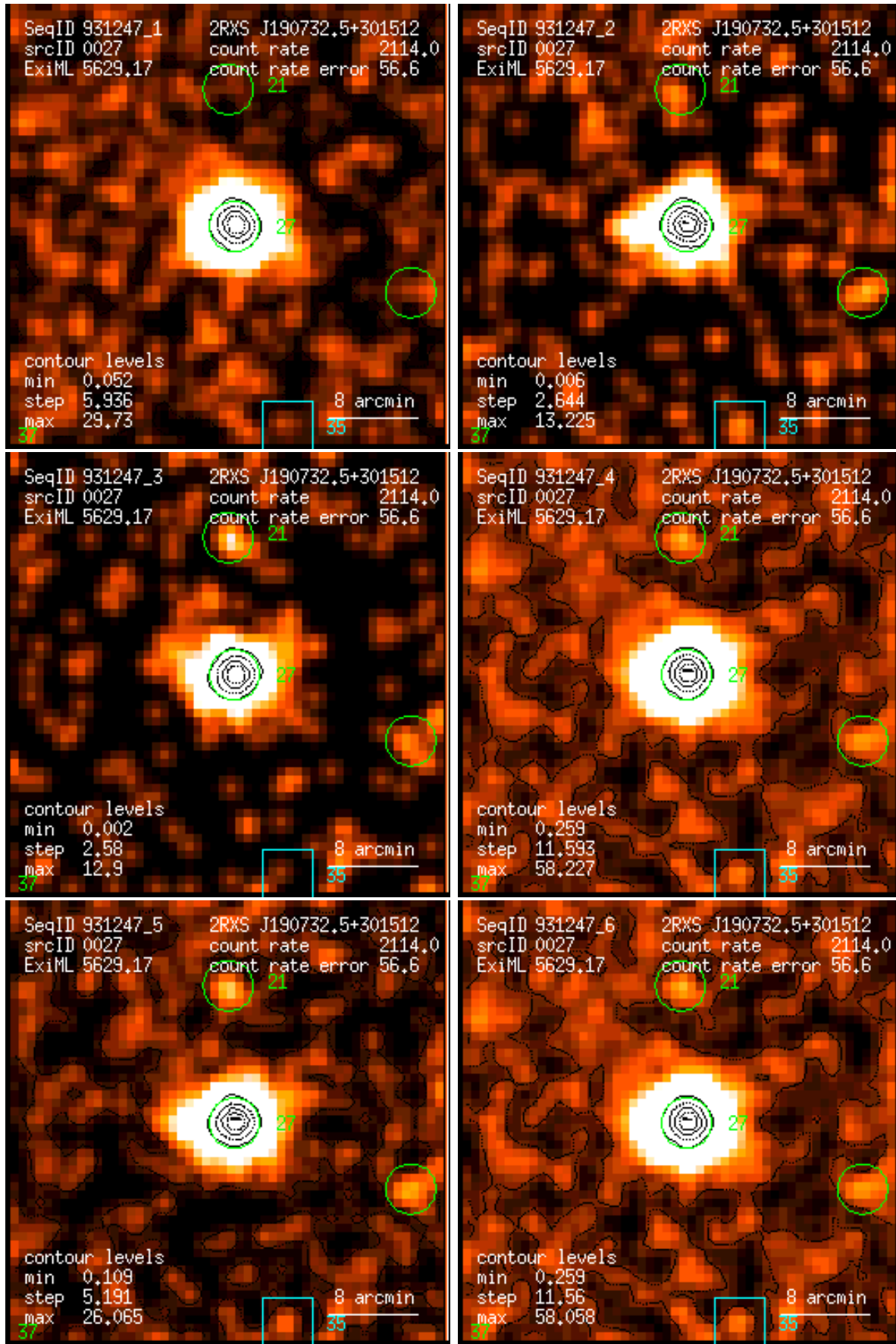
Figure 27: RASS 931247: detection 0027: band rate images, Gaussian filter: (1) PSPC channels 11 – 41, (2) 52 – 90, (3) 91 – 201, (4) 11 – 235, (5) 52 – 201, (6) 11 – 201. Broad band rates in counts/ks. Band rate contour levels in counts/ks/arcmin 2 .
