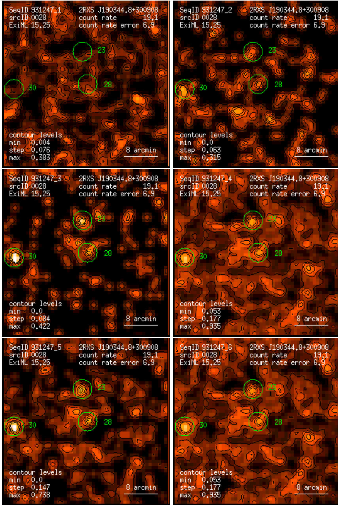
Figure 28: RASS 931247: detection 0028: band rate images, Gaussian filter: (1) PSPC channels 11 – 41, (2) 52 – 90, (3) 91 – 201, (4) 11 – 235, (5) 52 – 201, (6) 11 – 201. Broad band rates in counts/ks. Band rate contour levels in counts/ks/arcmin 2 .
