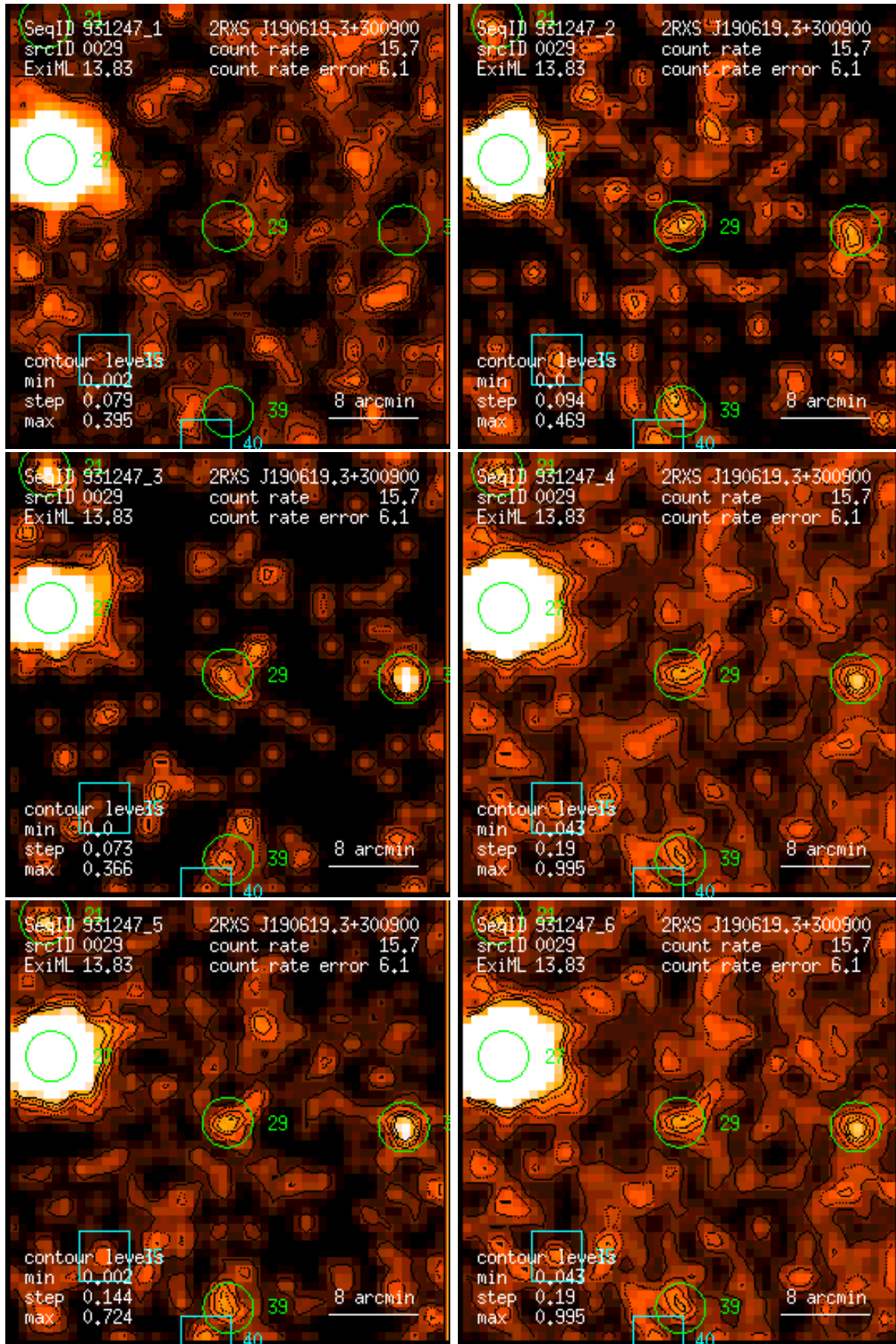
Figure 29: RASS 931247: detection 0029: band rate images, Gaussian filter: (1) PSPC channels 11 – 41, (2) 52 – 90, (3) 91 – 201, (4) 11 – 235, (5) 52 – 201, (6) 11 – 201. Broad band rates in counts/ks. Band rate contour levels in counts/ks/arcmin 2 .
