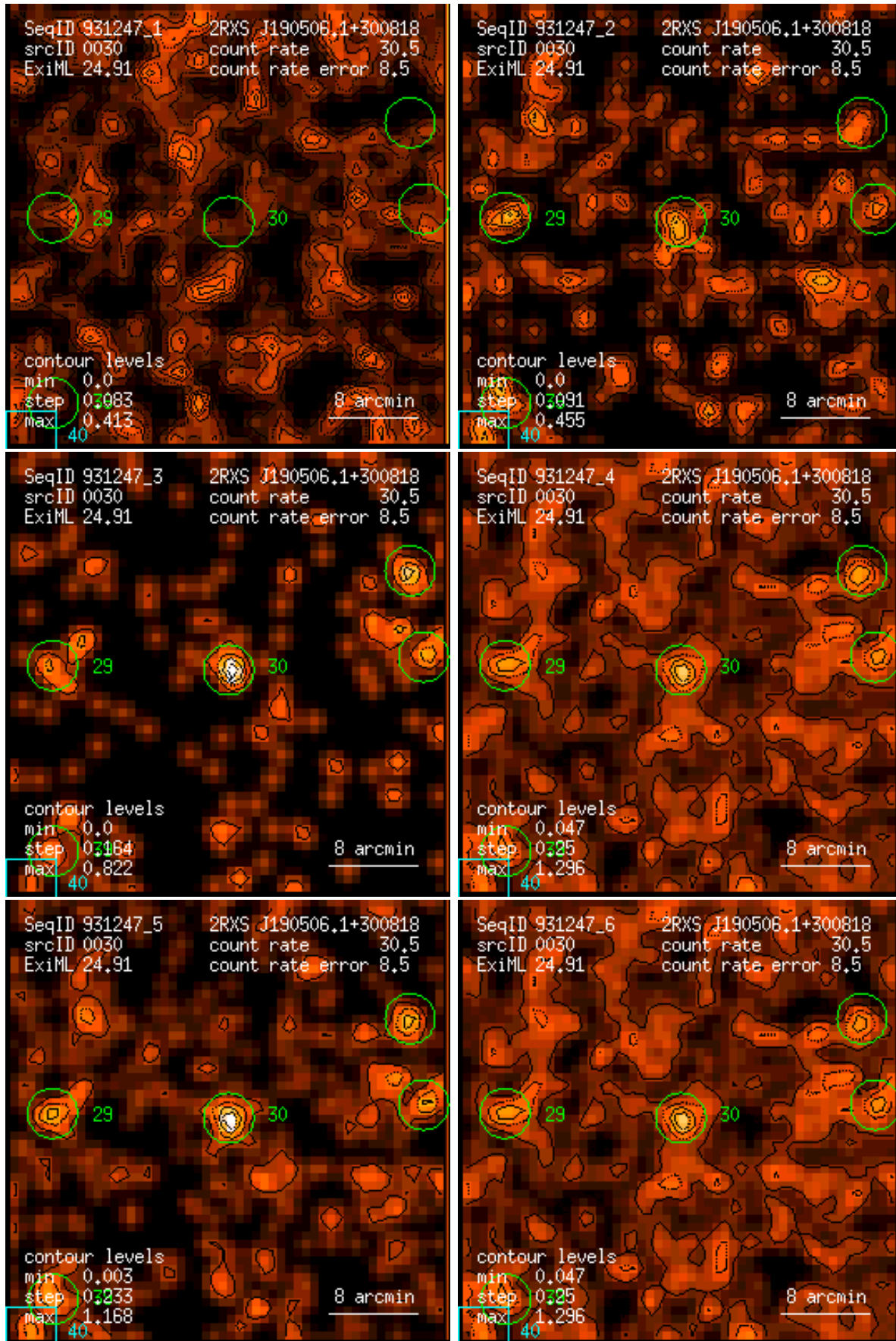
Figure 30: RASS 931247: detection 0030: band rate images, Gaussian filter: (1) PSPC channels 11 – 41, (2) 52 – 90, (3) 91 – 201, (4) 11 – 235, (5) 52 – 201, (6) 11 – 201. Broad band rates in counts/ks. Band rate contour levels in counts/ks/arcmin 2 .
