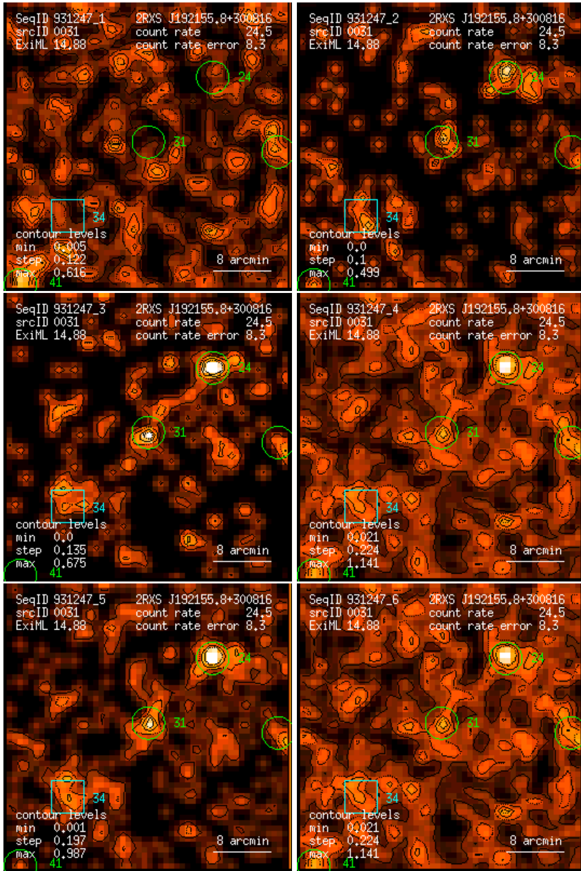
Figure 31: RASS 931247: detection 0031: band rate images, Gaussian filter: (1) PSPC channels 11 – 41, (2) 52 – 90, (3) 91 – 201, (4) 11 – 235, (5) 52 – 201, (6) 11 – 201. Broad band rates in counts/ks. Band rate contour levels in counts/ks/arcmin 2 .
