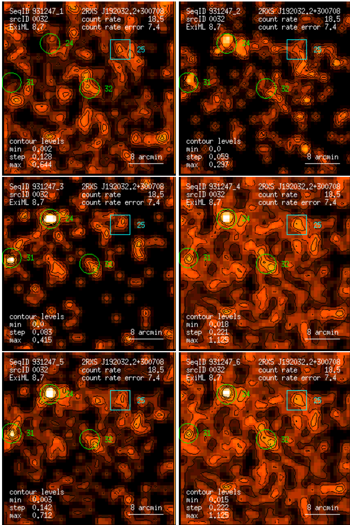
Figure 32: RASS 931247: detection 0032: band rate images, Gaussian filter: (1) PSPC channels 11 – 41, (2) 52 – 90, (3) 91 – 201, (4) 11 – 235, (5) 52 – 201, (6) 11 – 201. Broad band rates in counts/ks. Band rate contour levels in counts/ks/arcmin 2 .
