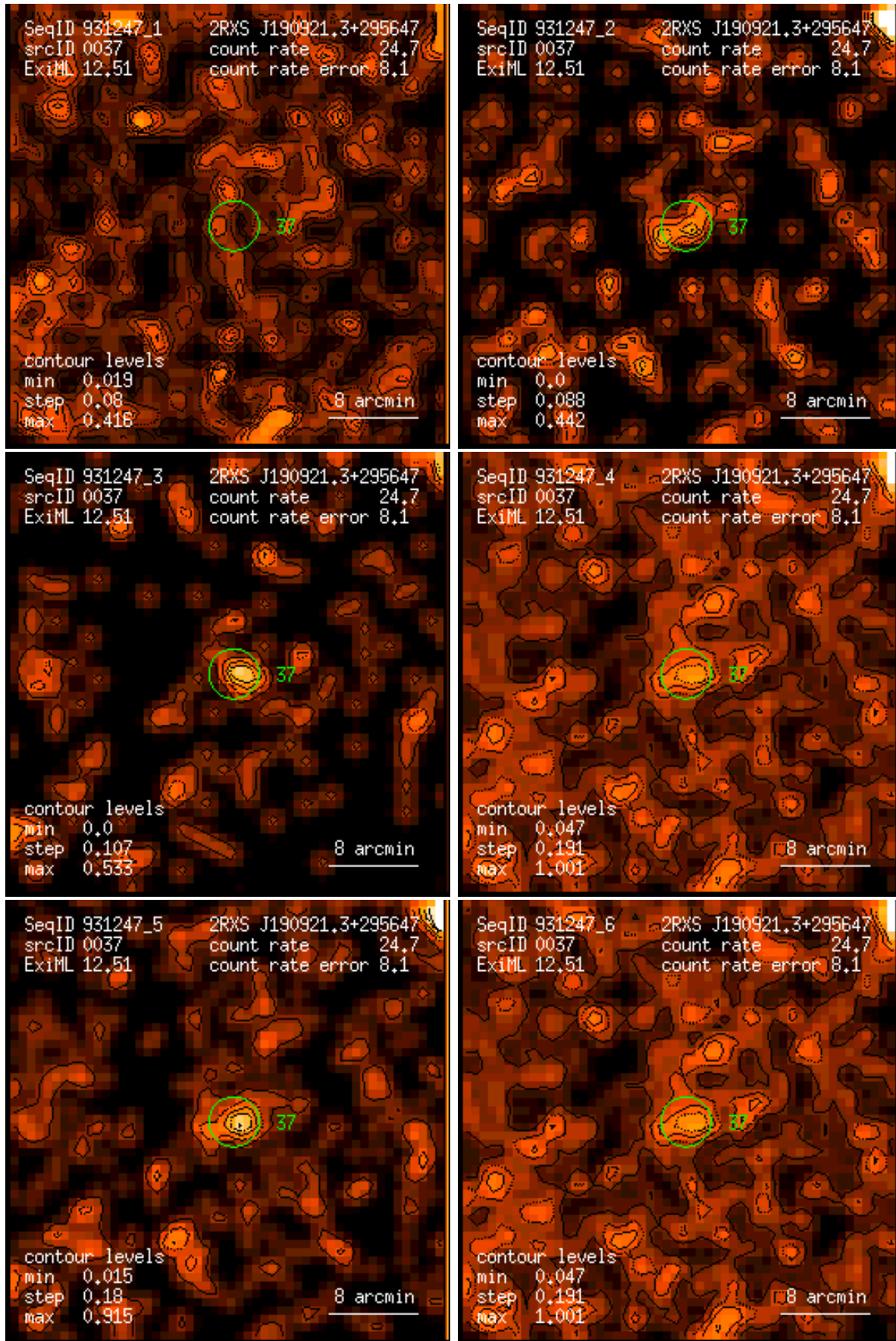
Figure 37: RASS 931247: detection 0037: band rate images, Gaussian filter: (1) PSPC channels 11 – 41, (2) 52 – 90, (3) 91 – 201, (4) 11 – 235, (5) 52 – 201, (6) 11 – 201. Broad band rates in counts/ks. Band rate contour levels in counts/ks/arcmin 2 .
