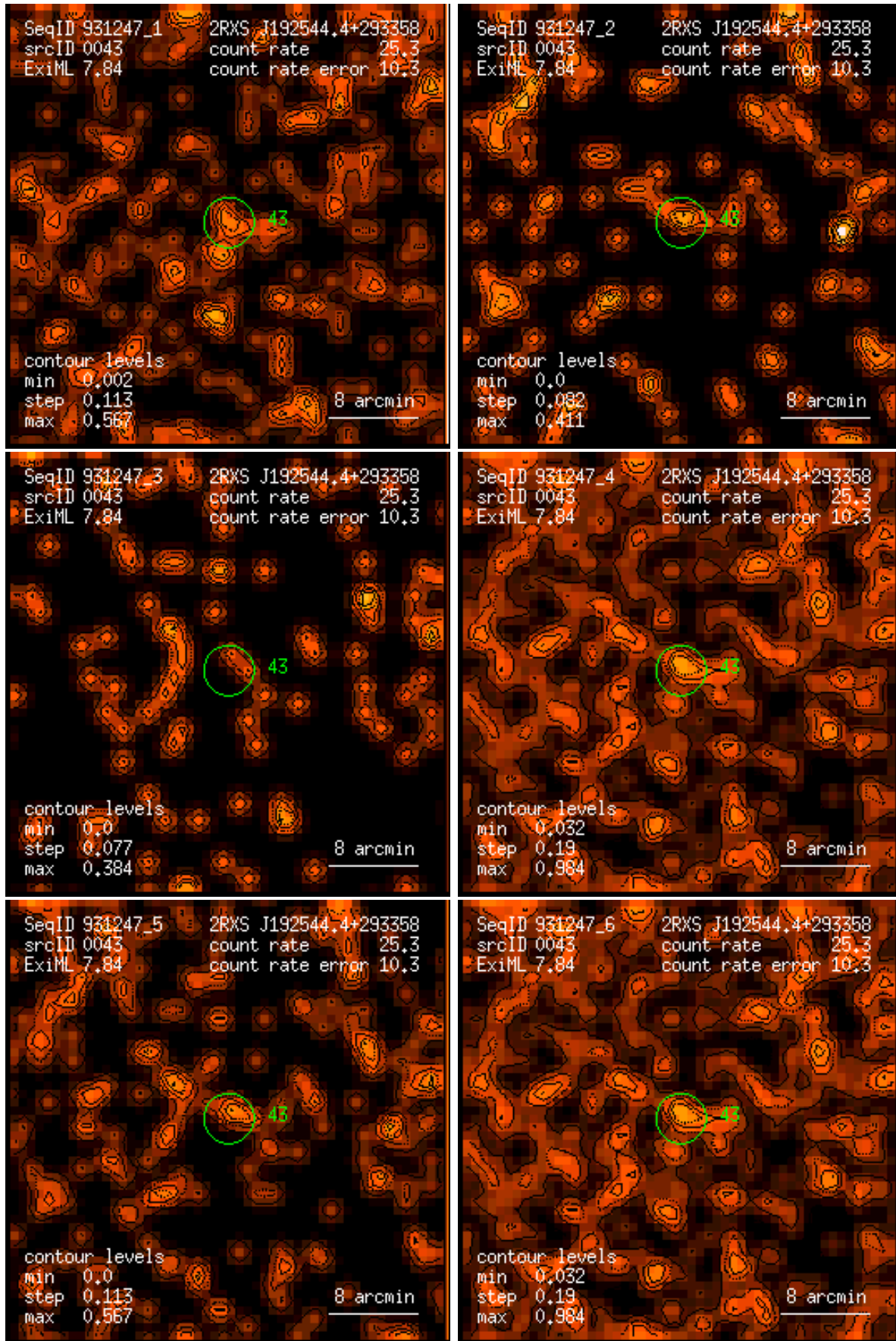
Figure 43: RASS 931247: detection 0043: band rate images, Gaussian filter: (1) PSPC channels 11 – 41, (2) 52 – 90, (3) 91 – 201, (4) 11 – 235, (5) 52 – 201, (6) 11 – 201. Broad band rates in counts/ks. Band rate contour levels in counts/ks/arcmin 2 .
