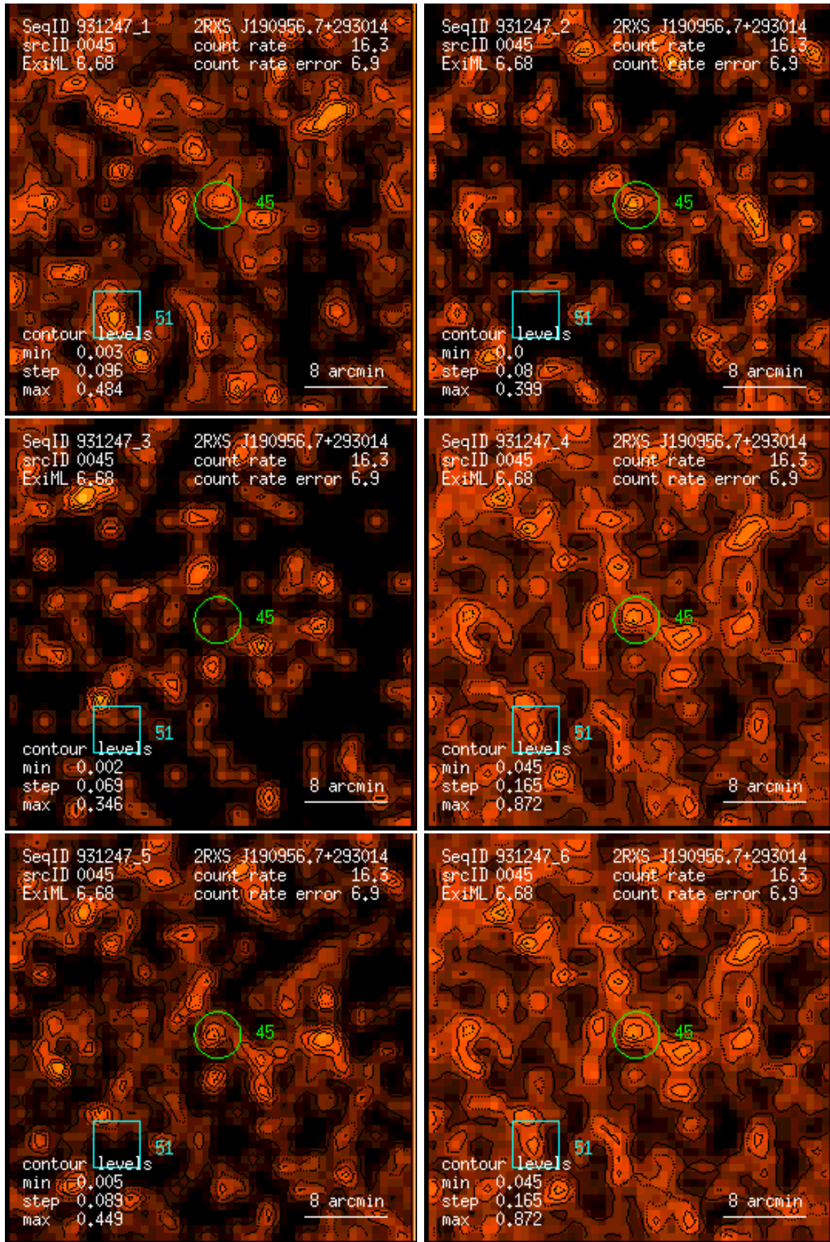
Figure 45: RASS 931247: detection 0045: band rate images, Gaussian filter: (1) PSPC channels 11 – 41, (2) 52 – 90, (3) 91 – 201, (4) 11 – 235, (5) 52 – 201, (6) 11 – 201. Broad band rates in counts/ks. Band rate contour levels in counts/ks/arcmin 2 .
