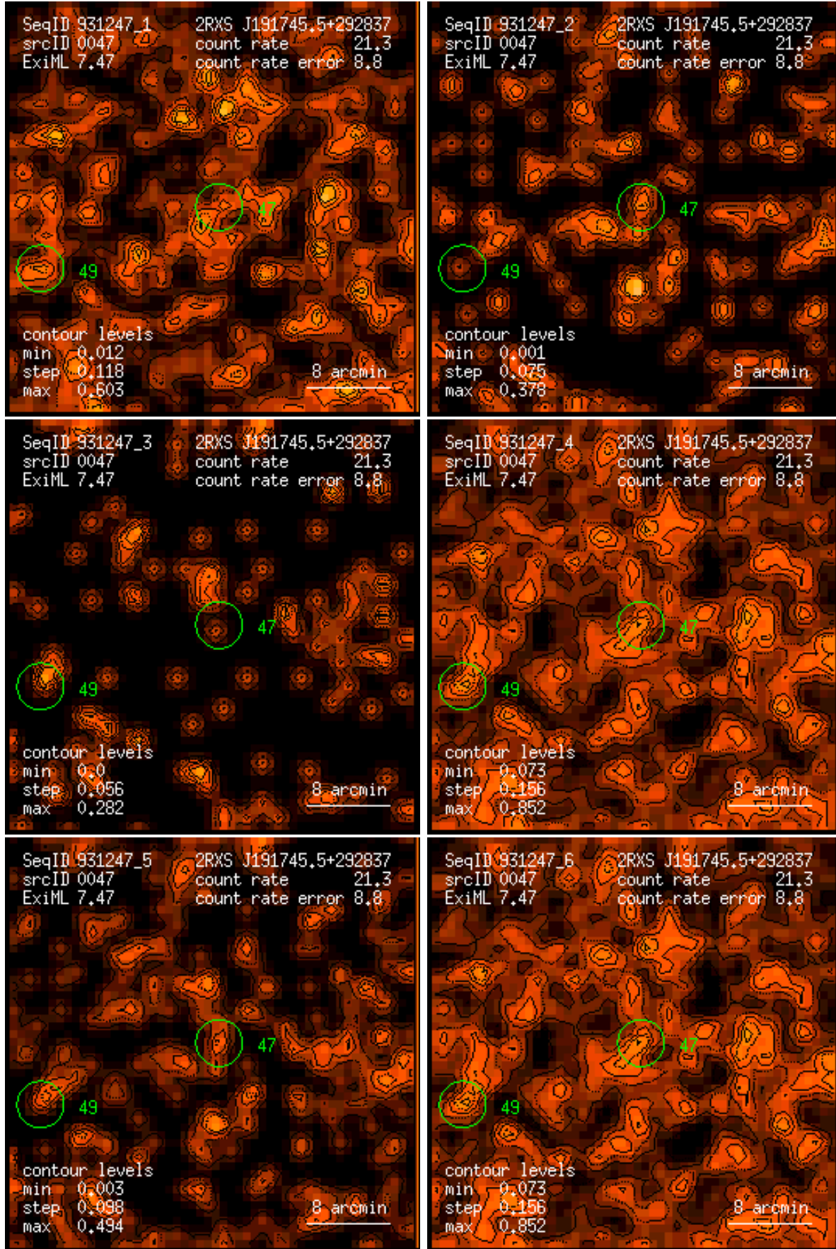
Figure 47: RASS 931247: detection 0047: band rate images, Gaussian filter: (1) PSPC channels 11 – 41, (2) 52 – 90, (3) 91 – 201, (4) 11 – 235, (5) 52 – 201, (6) 11 – 201. Broad band rates in counts/ks. Band rate contour levels in counts/ks/arcmin 2 .
