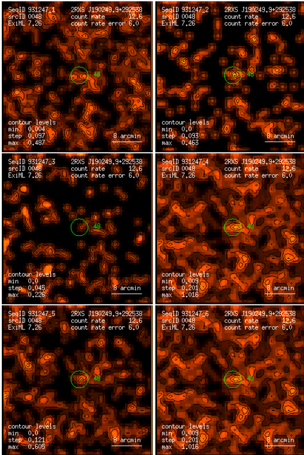
Figure 48: RASS 931247: detection 0048: band rate images, Gaussian filter: (1) PSPC channels 11 – 41, (2) 52 – 90, (3) 91 – 201, (4) 11 – 235, (5) 52 – 201, (6) 11 – 201. Broad band rates in counts/ks. Band rate contour levels in counts/ks/arcmin 2 .
