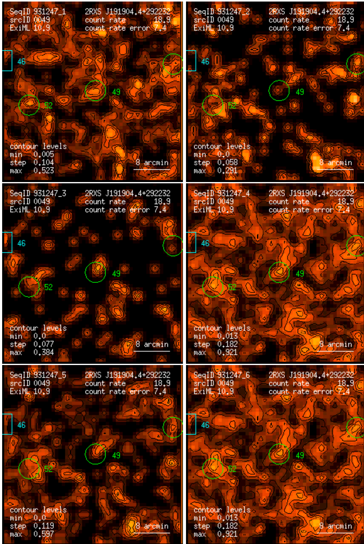
Figure 49: RASS 931247: detection 0049: band rate images, Gaussian filter: (1) PSPC channels 11 – 41, (2) 52 – 90, (3) 91 – 201, (4) 11 – 235, (5) 52 – 201, (6) 11 – 201. Broad band rates in counts/ks. Band rate contour levels in counts/ks/arcmin 2 .
