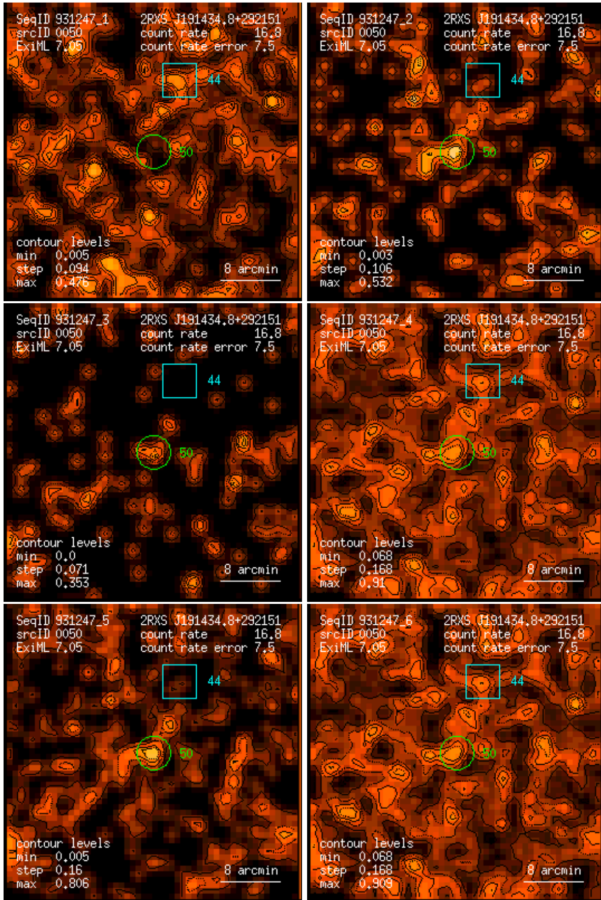
Figure 50: RASS 931247: detection 0050: band rate images, Gaussian filter: (1) PSPC channels 11 – 41, (2) 52 – 90, (3) 91 – 201, (4) 11 – 235, (5) 52 – 201, (6) 11 – 201. Broad band rates in counts/ks. Band rate contour levels in counts/ks/arcmin 2 .
