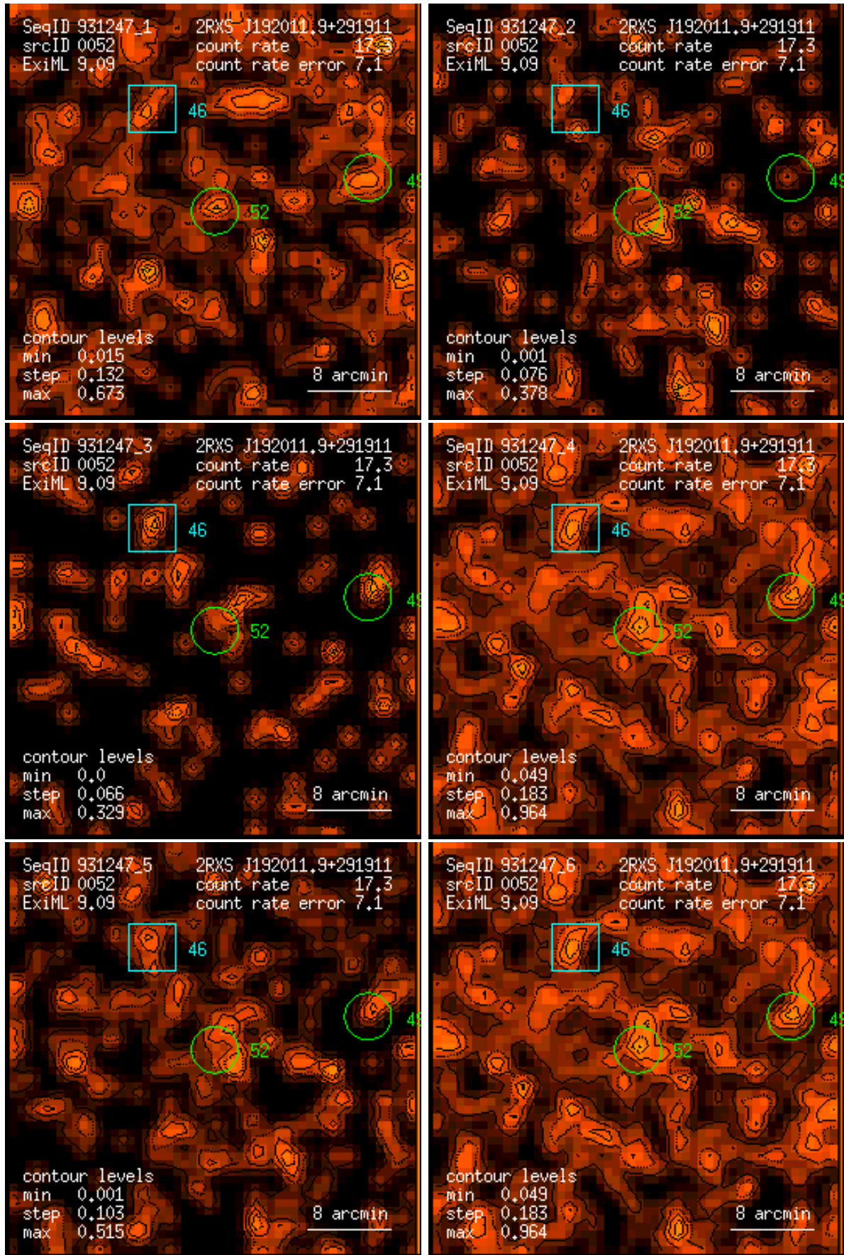
Figure 52: RASS 931247: detection 0052: band rate images, Gaussian filter: (1) PSPC channels 11 – 41, (2) 52 – 90, (3) 91 – 201, (4) 11 – 235, (5) 52 – 201, (6) 11 – 201. Broad band rates in counts/ks. Band rate contour levels in counts/ks/arcmin 2 .
