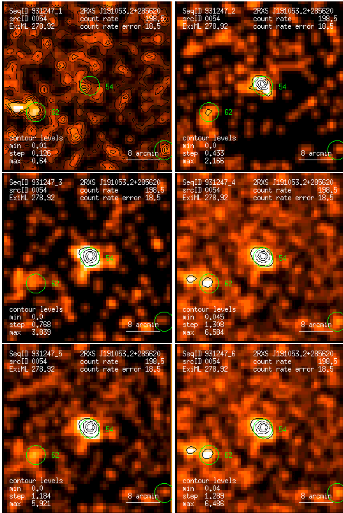
Figure 54: RASS 931247: detection 0054: band rate images, Gaussian filter: (1) PSPC channels 11 – 41, (2) 52 – 90, (3) 91 – 201, (4) 11 – 235, (5) 52 – 201, (6) 11 – 201. Broad band rates in counts/ks. Band rate contour levels in counts/ks/arcmin 2 .
