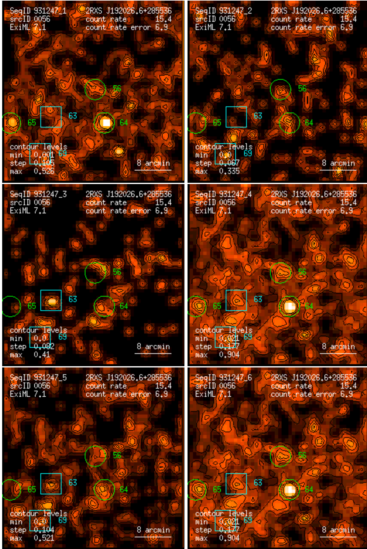
Figure 56: RASS 931247: detection 0056: band rate images, Gaussian filter: (1) PSPC channels 11 – 41, (2) 52 – 90, (3) 91 – 201, (4) 11 – 235, (5) 52 – 201, (6) 11 – 201. Broad band rates in counts/ks. Band rate contour levels in counts/ks/arcmin 2 .
