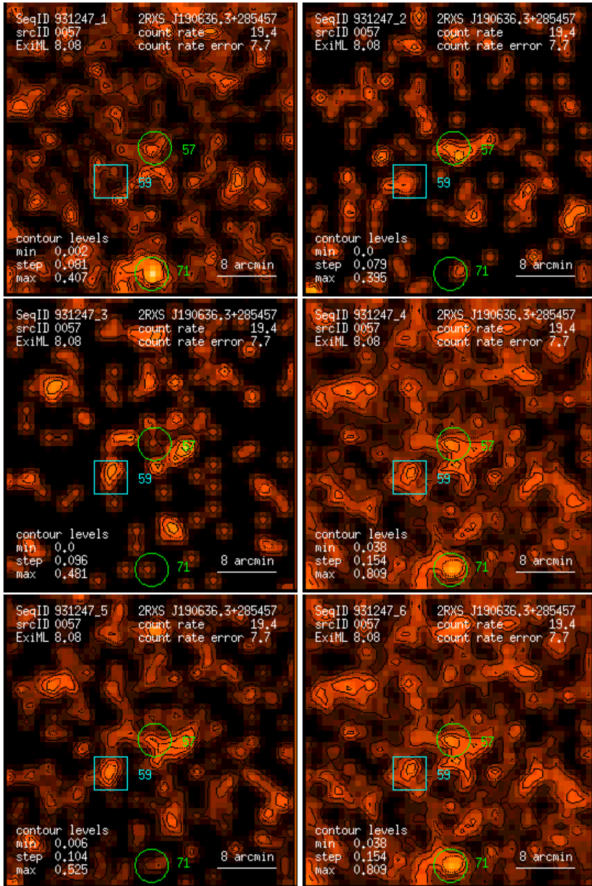
Figure 57: RASS 931247: detection 0057: band rate images, Gaussian filter: (1) PSPC channels 11 – 41, (2) 52 – 90, (3) 91 – 201, (4) 11 – 235, (5) 52 – 201, (6) 11 – 201. Broad band rates in counts/ks. Band rate contour levels in counts/ks/arcmin 2 .
