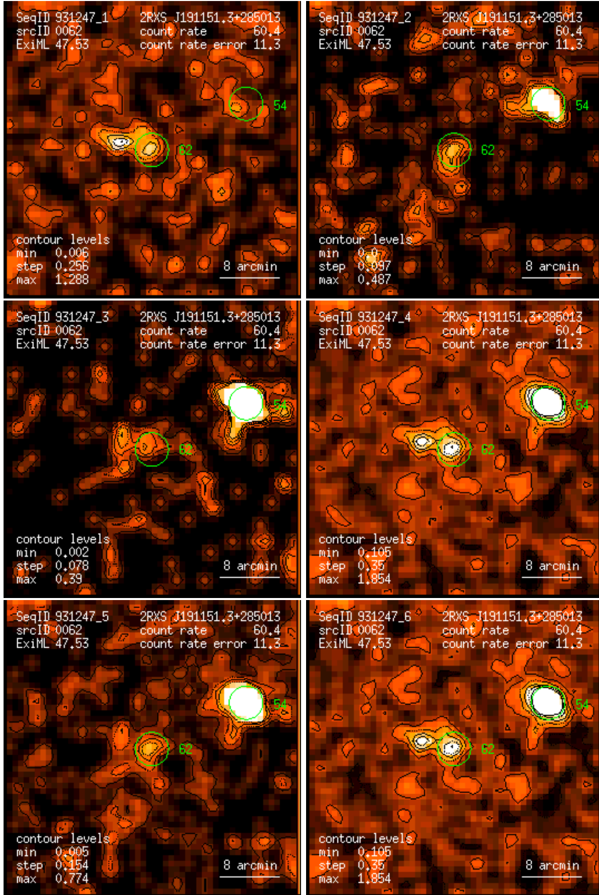
Figure 62: RASS 931247: detection 0062: band rate images, Gaussian filter: (1) PSPC channels 11 – 41, (2) 52 – 90, (3) 91 – 201, (4) 11 – 235, (5) 52 – 201, (6) 11 – 201. Broad band rates in counts/ks. Band rate contour levels in counts/ks/arcmin 2 .
