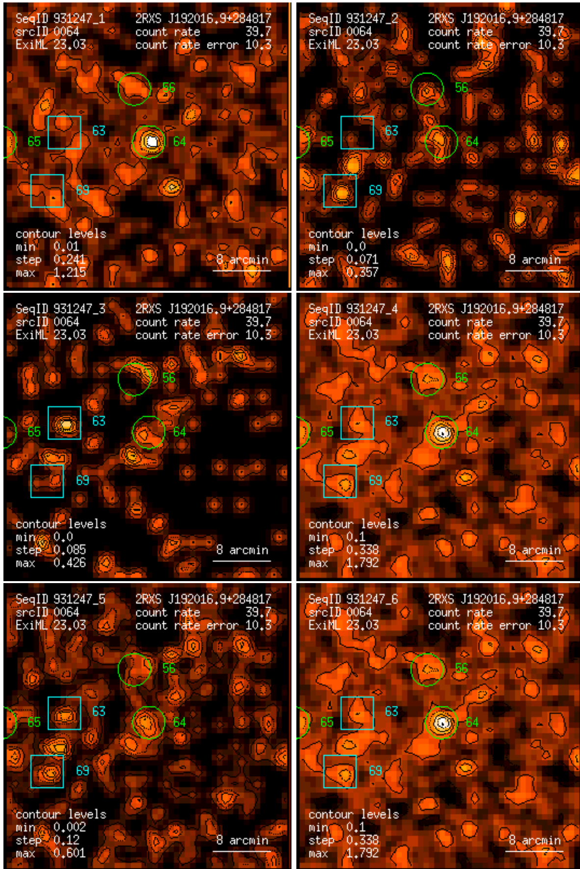
Figure 64: RASS 931247: detection 0064: band rate images, Gaussian filter: (1) PSPC channels 11 – 41, (2) 52 – 90, (3) 91 – 201, (4) 11 – 235, (5) 52 – 201, (6) 11 – 201. Broad band rates in counts/ks. Band rate contour levels in counts/ks/arcmin 2 .
