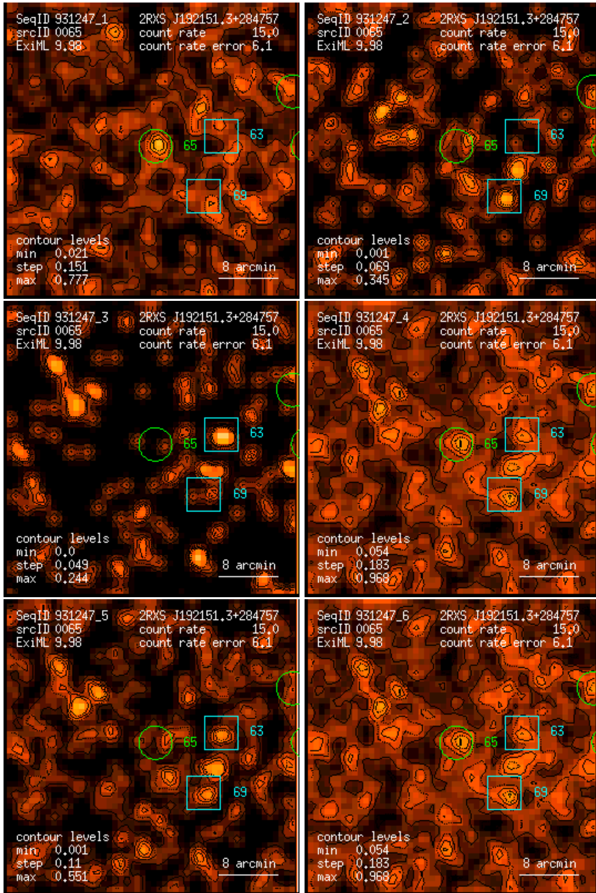
Figure 65: RASS 931247: detection 0065: band rate images, Gaussian filter: (1) PSPC channels 11 – 41, (2) 52 – 90, (3) 91 – 201, (4) 11 – 235, (5) 52 – 201, (6) 11 – 201. Broad band rates in counts/ks. Band rate contour levels in counts/ks/arcmin 2 .
