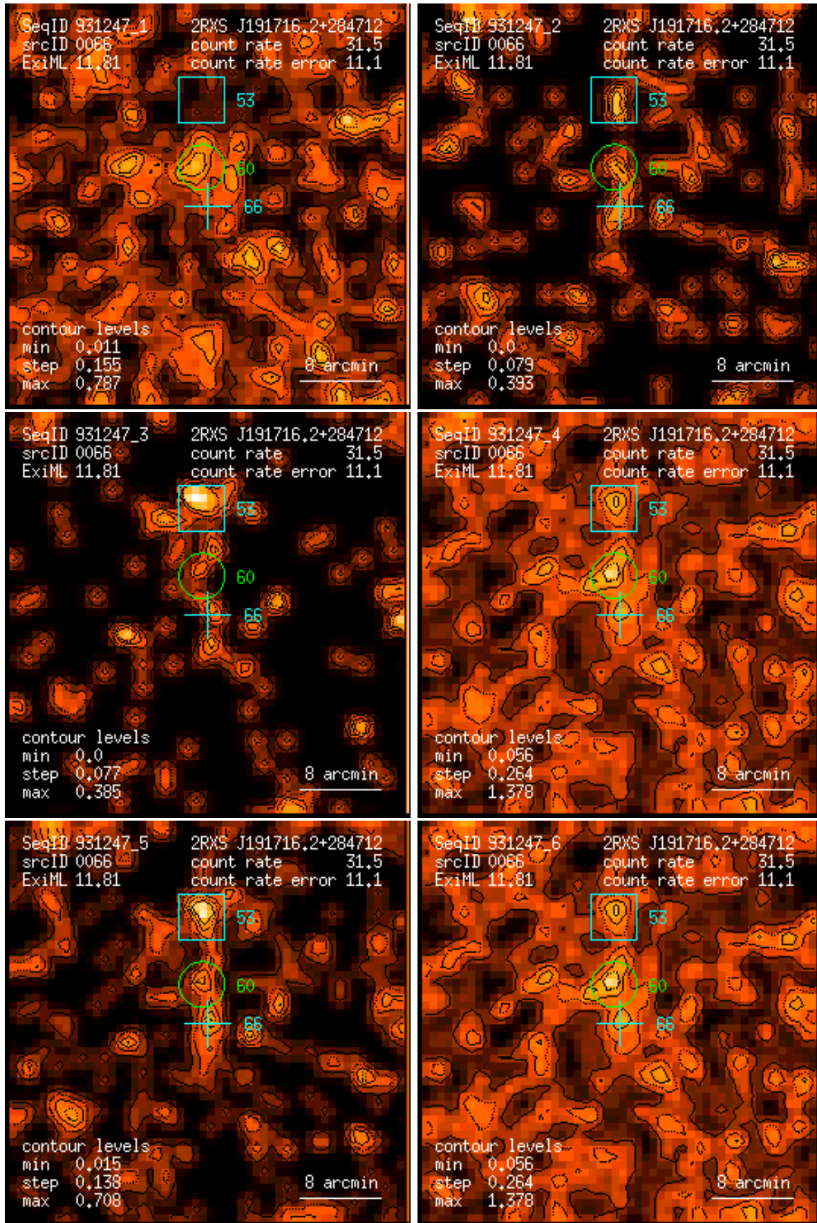
Figure 66: RASS 931247: detection 0066: band rate images, Gaussian filter: (1) PSPC channels 11 – 41, (2) 52 – 90, (3) 91 – 201, (4) 11 – 235, (5) 52 – 201, (6) 11 – 201. Broad band rates in counts/ks. Band rate contour levels in counts/ks/arcmin 2 .
