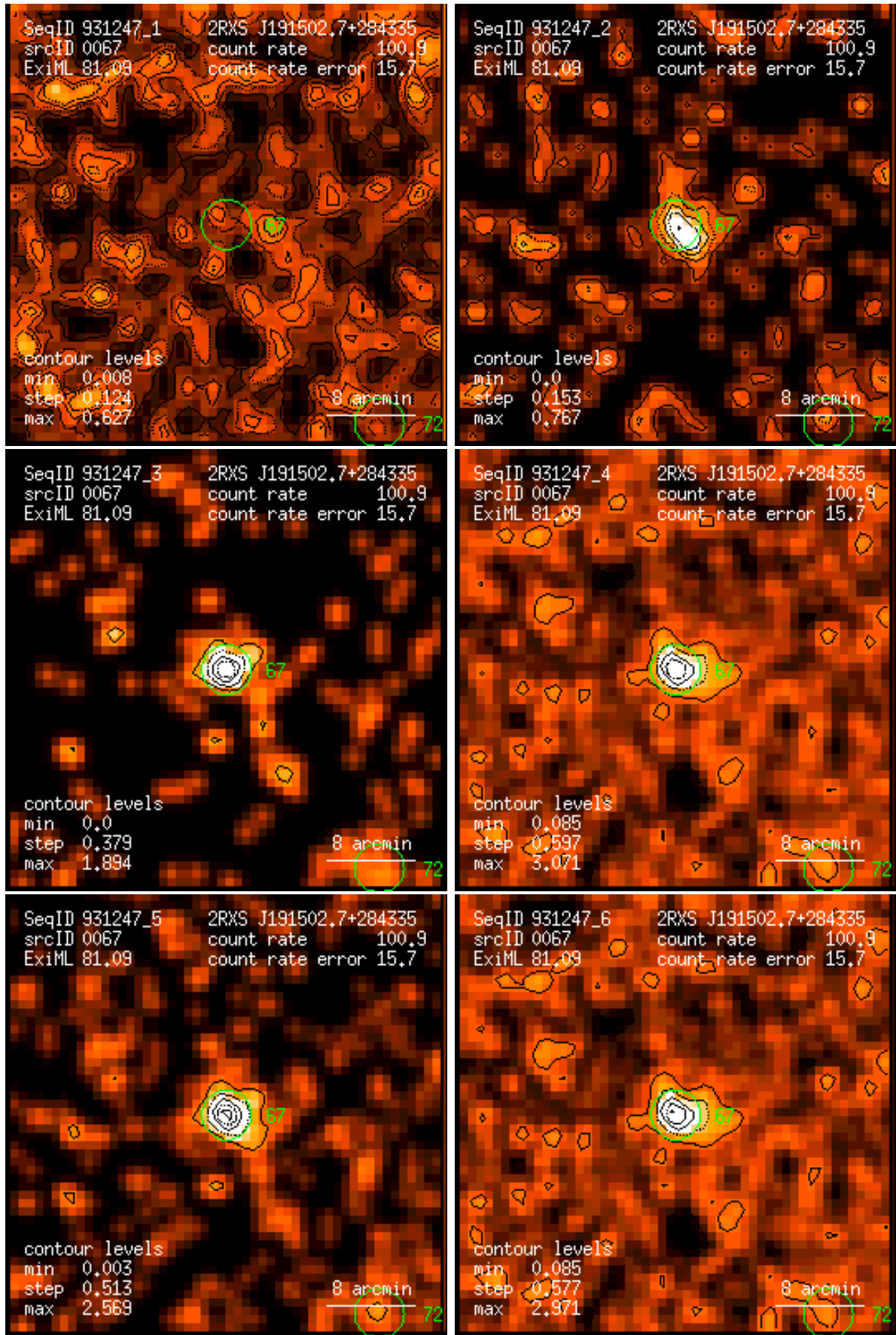
Figure 67: RASS 931247: detection 0067: band rate images, Gaussian filter: (1) PSPC channels 11 – 41, (2) 52 – 90, (3) 91 – 201, (4) 11 – 235, (5) 52 – 201, (6) 11 – 201. Broad band rates in counts/ks. Band rate contour levels in counts/ks/arcmin 2 .
