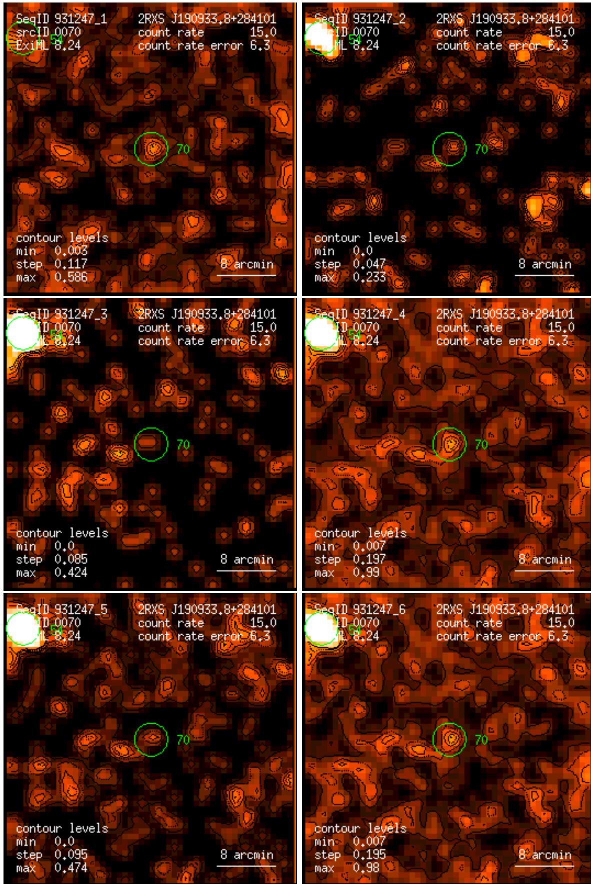
Figure 70: RASS 931247: detection 0070: band rate images, Gaussian filter: (1) PSPC channels 11 – 41, (2) 52 – 90, (3) 91 – 201, (4) 11 – 235, (5) 52 – 201, (6) 11 – 201. Broad band rates in counts/ks. Band rate contour levels in counts/ks/arcmin 2 .
